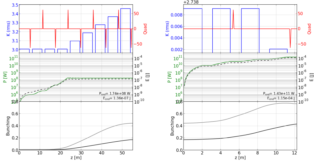
Fig. 3. Electron beam and radiation parameters evolution within planar (left sub-figure) and helical (right sub-figure) undulators for 2000 eV photon energy. Top subplots represent undulator K values and quadrupole fields. Next subplots provide the radiation peak power and integrated energy of the pulse as a function of the undulator length. Last subplots show the evolution of a maximum (black line) and average (grey line) bunching along the beam
