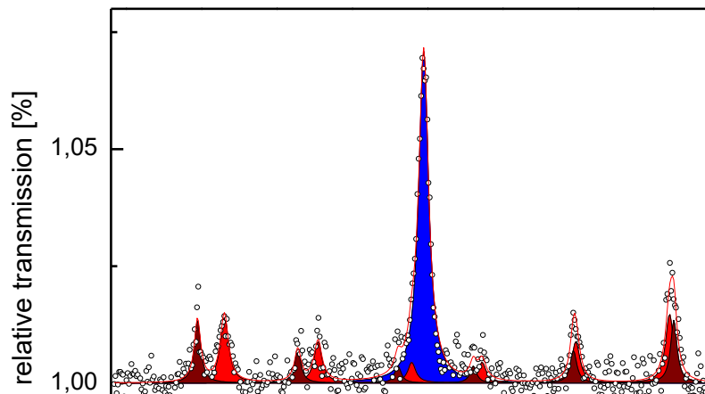
Fig.1. MS spectrum of sample 1. Dark red component represents A-sites of magnetite (Sextet A), red component represents B-sites of magnetite (Sextet B), blue component represents austenitic base material of the feed water dispersion box.
