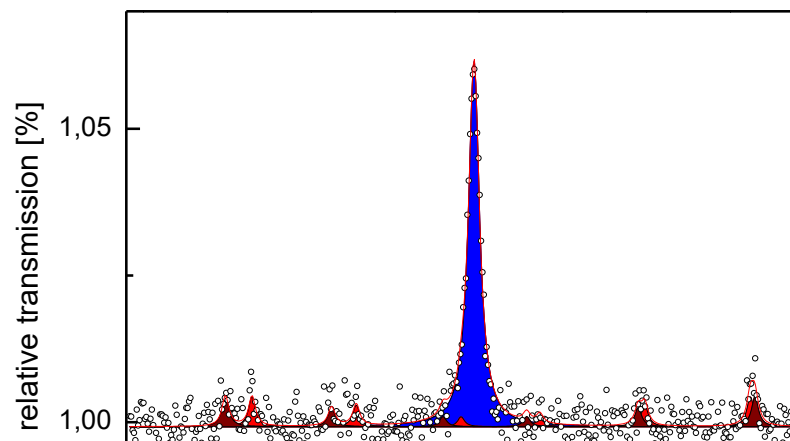
Fig.2. MS spectrum of sample 2. Dark red component represents A-sites of magnetite (Sextet A), red component represents B-sites of magnetite (Sextet B), blue component represents austenitic base material of the feed water dispersion box.
