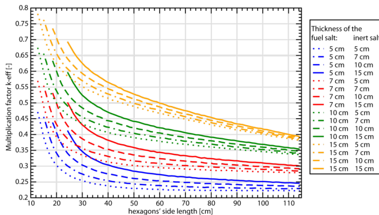
FIG. 9. Variation of the multiplication factor as a function of the hexagon side length.
