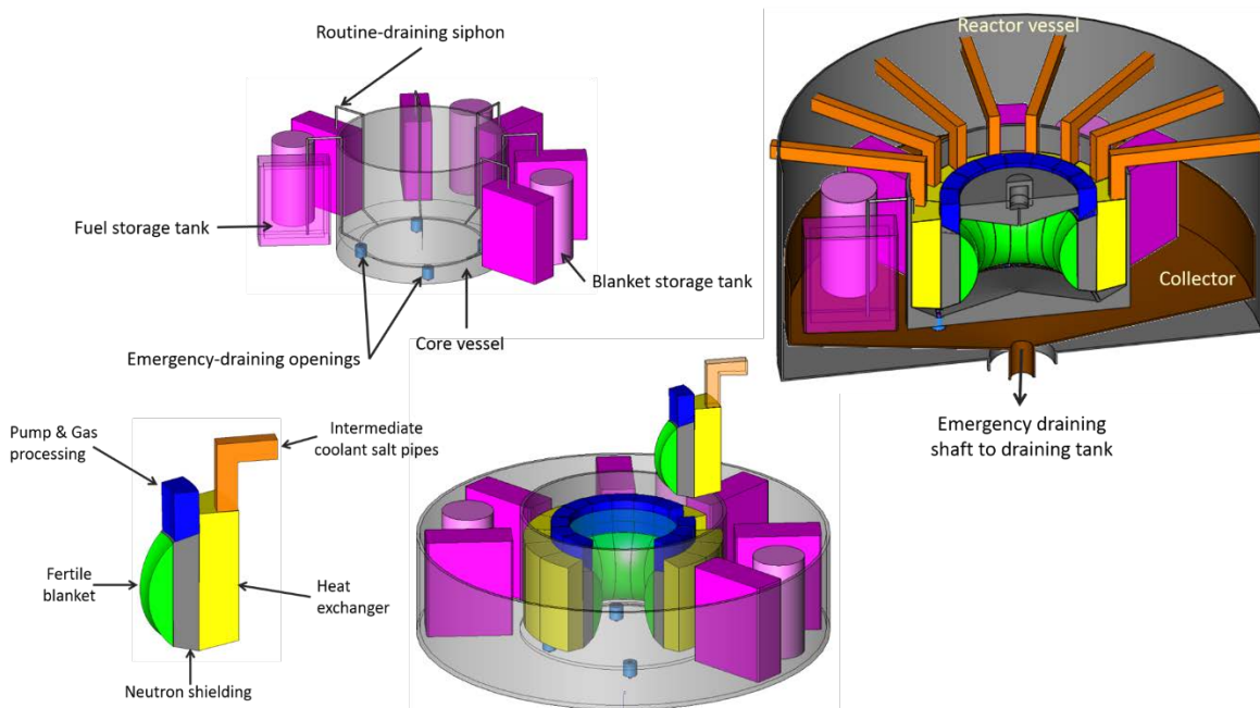
FIG. 2. Schematic representation of a cooling sector (bottom left), cooling sector arrangement in the core vessel (bottom right), storage tank arrangement around the core vessel (top left), and reactor vessel (top right).
