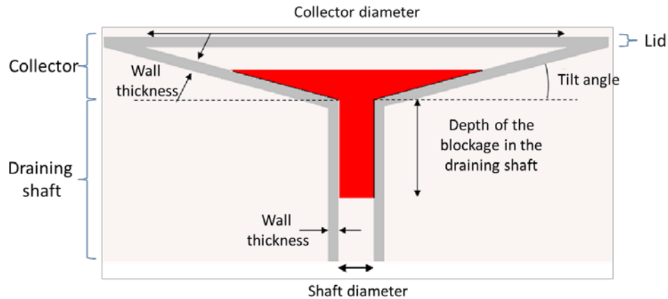
FIG. 7. Schematic drawing of the collector and draining shaft
