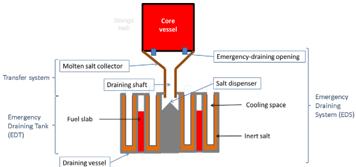
FIG. 3. Schematic overall representation of the draining system - vertical cross-section
