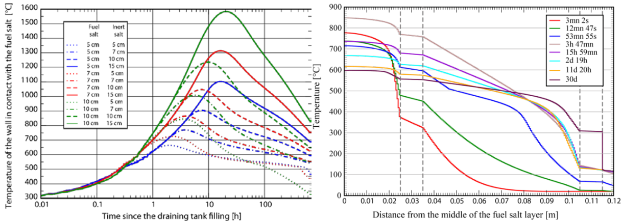
FIG. 5. Time evolution of the temperature of the metallic wall in contact with the fuel salt (left) and Temperature spatial distribution for the "5cm fuel salt and 7cm inert salt" case after various cooling times (right).
