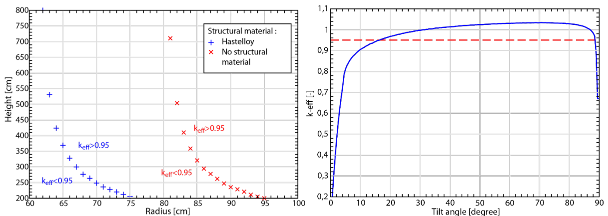
FIG. 8. Height of the draining shaft as a function of its radius for a multiplication factor of 0.95 (left) and multiplication factor as a function of the tilt angle of the collector (right).
