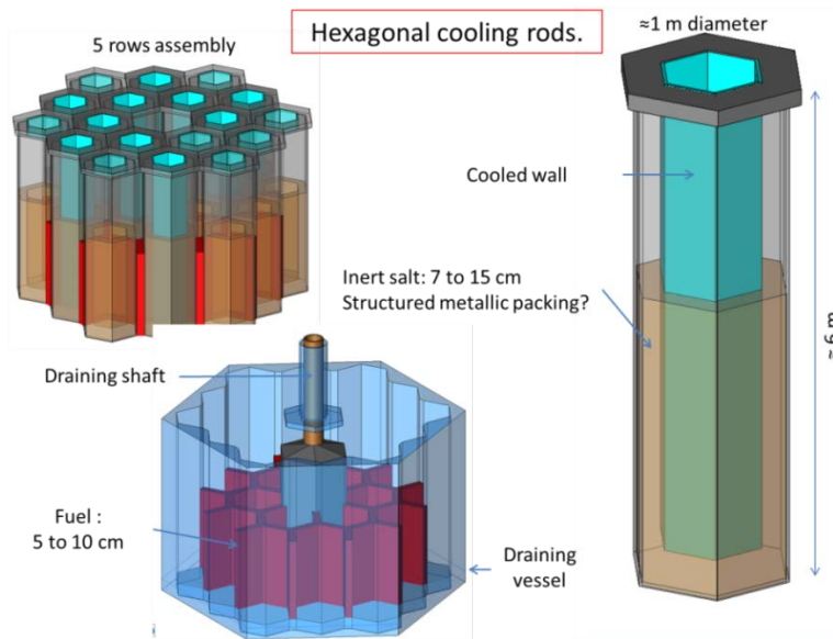
FIG. 4. The emergency-draining tank (hexagonal version) is composed of a thick metallic casing (blue) containing cooling rods (center) between which the fuel salt (red) spreads. Below, these cooling rods are removed to show the fuel salt and the partition inert block.
