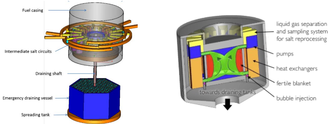
FIG. 1. Schematic view of the MSFR fuel circuit and emergency draining tank (left) and zoom on the fuel circuit (right).
