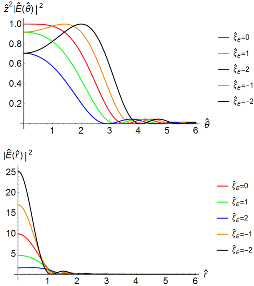
Fig. 2. Top panel: the function z^2 |\hat{E}(\hat{\theta})|^2 is plot for different values of \hat{\xi}_E . Bottom panel: the function |\hat{E}(\hat{r})|^2 is plot for different values of \hat{\xi}_E . Both functions are axis-symmetric, i.e. a 3D picture can be obtained by a rotation around the vertical axis. Here \hat{l} = \mathbf{0} and \hat{\eta} = \mathbf{0} .
