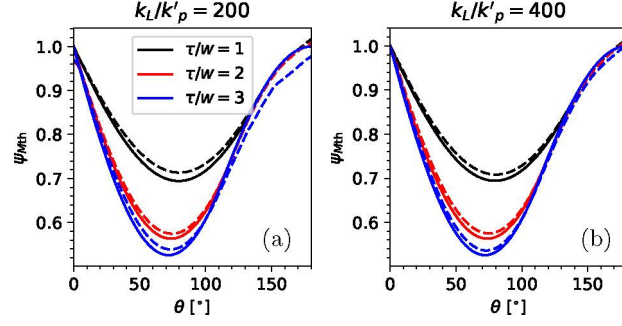
FIG. 2: Verification of the ponderomotive scattering model by PIC simulations. The threshold of \psi_M for trapping to occur ( \psi_{M\text{th}} ) vs. \theta (the angle between z and z' ) is plotted for the model (solid curves) and for the PIC simulations (dashed curves). The black, red and blue colors indicate different pulse durations. Two relative frequencies k_L/k'_p = 200 (a) and 400 (b) are considered.
