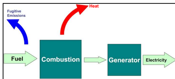
Figure 1. The Typical Process Scheme for Power Plants in Batam [9] Source: EMEP/EEA Emission Inventory Guidebook 2013, Fig. 2-2, Chapter 1.
