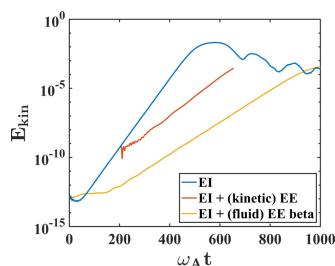
Figure 6: Kinetic energy evolution of energetic ion (EI) driven TAE with the effect of energetic electrons (EEs).
