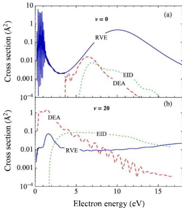
Fig. 1. Summary on electron- \text{O}_2 cross sections [5]: vibrational excitation (RVE), dissociative attachment (DEA), and dissociative excitation (EID) processes for the vibrational levels v = 0 (a) and v = 20 (b).
