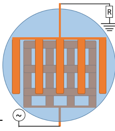
Top-view of upper electrode
