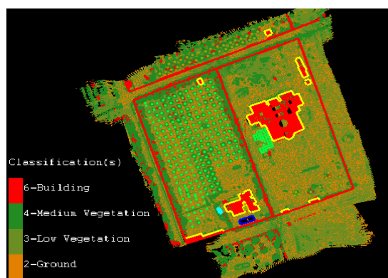
Figure 5. The restitution superimposed on the Lidar point cloud
