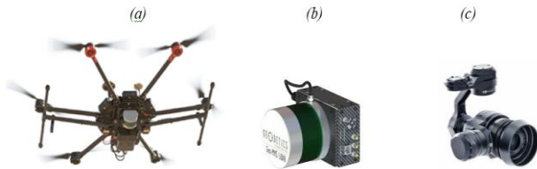
Figure 2. Equipment: (a) Drone DJI Matrice 600 Pro, (b) LiDAR Geo-MMS, (c) Camera ZENMUSE X5
