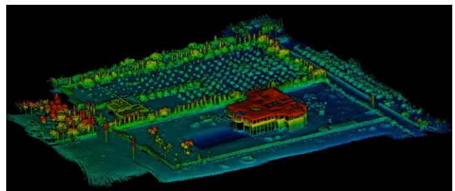
Figure 3. Point cloud of the study area obtained by Drone-based LiDAR
