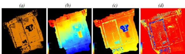
Figure 4. Processing Results of LiDAR Data: (a) Classification, (b) DTM, (c) DSM, (d) DCM
