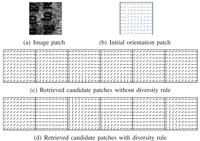
Fig. 10. Candidate orientation patches obtained without (c) and with (d) diversity rule.
