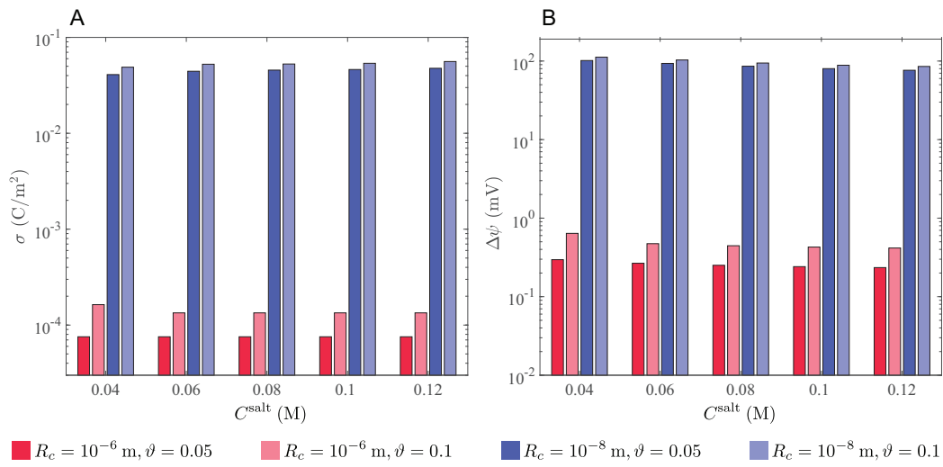
Figure S4: Stability limits along steady-state solution branches of Fig 3 in the positive orthant. (A) surface-charge density, at which stability is lost. (B) Membrane potential, at which stability is lost.
