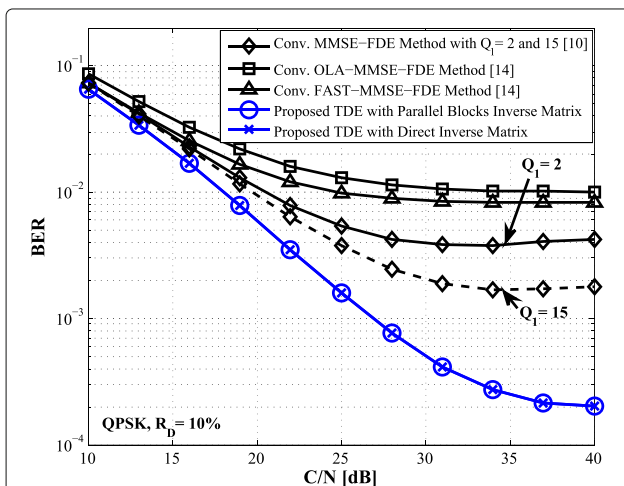
Fig. 7 BER performances versus C/N for proposed TDE and conventional FDE methods with low-complexity reduction algorithms when the modulation method is QPSK and R_D is 10%
