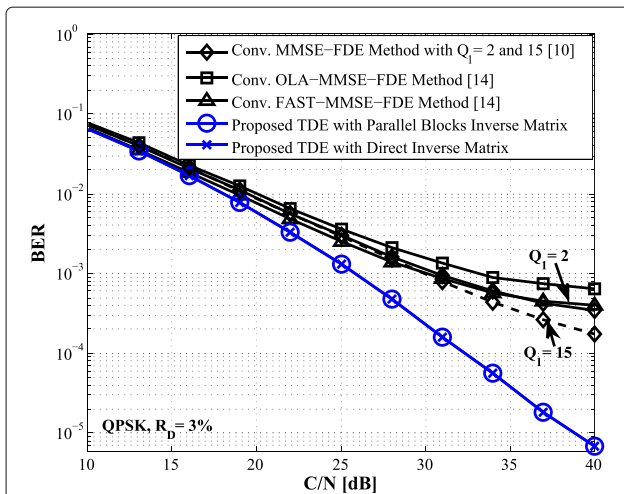
Fig. 6 BER performances versus C/N for proposed TDE and conventional FDE methods with low-complexity reduction algorithms when the modulation method is QPSK and R_D is 3%
