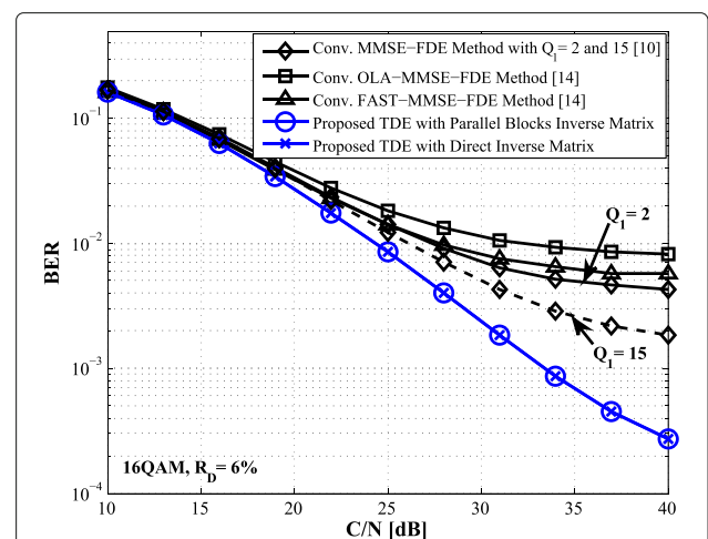
Fig. 8 BER performances versus C/N for proposed TDE and conventional FDE methods with low-complexity reduction algorithms when the modulation method is 16QAM and R_D is 6%
