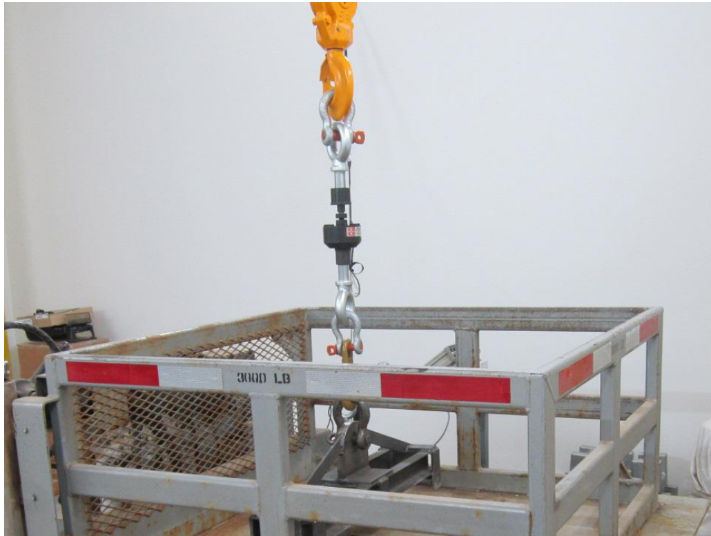
Morehouse Precision Calibration Load Cell with Custom Adapters
