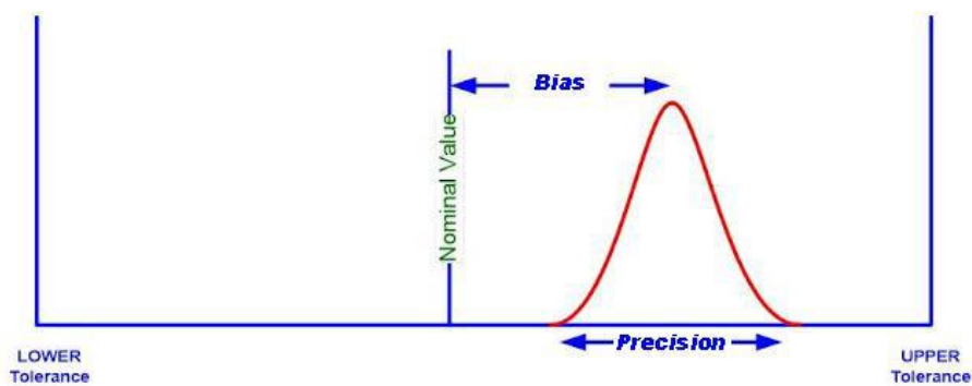
Figure 6: Accuracy
