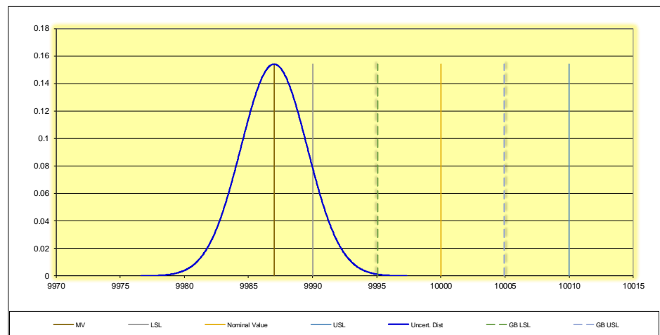
Figure 5: Graph Showing what happens if we do not correct for the + 9 N bias (1.93:1 TUR, which stays the same)
