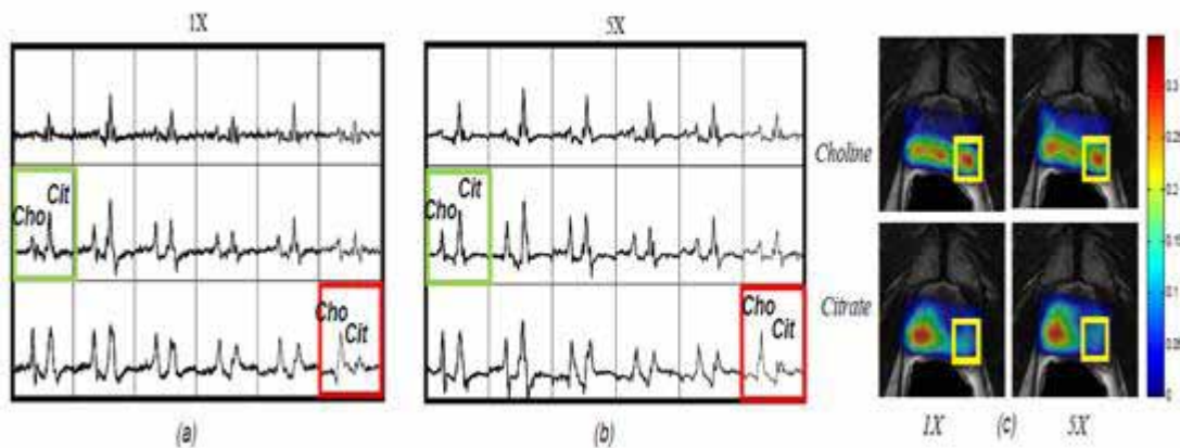
FIGURE 10. (a) Plot of the spectra of a representative prostate cancer MRSI at 1x (full k -space reconstruction); (b) an acceleration factor of 5 as compared to the original MRSI data (1x). Prostate cancer (shown in the red voxel) is characterized by increased choline (Cho) and reduced citrate (Cit) levels when compared to the metabolite profile of a normal prostate tissue (shown in green). (c) shows the Cho and Cit metabolite maps for the prostate cancer data at acceleration factors 1 and 5. The yellow boxes on the metabolite maps represent the location of the prostate cancer. 41
