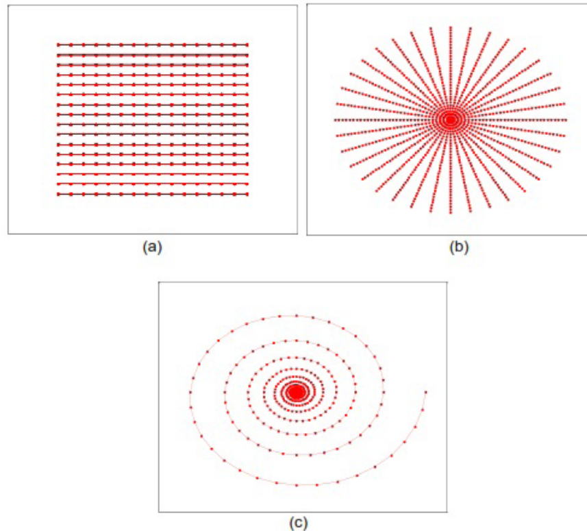
FIGURE 5. k -space trajectories: (a) Cartesian; (b) radial; (c) spiral with increased sampling in the center
