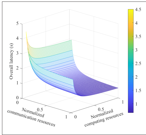
FIGURE 2. A schematic diagram of the overall latency of a single offloading task with different communication and computing resources provided.
