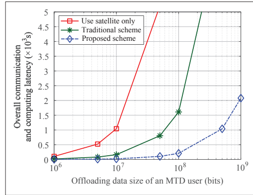
FIGURE 5. Latency comparison of different schemes.
