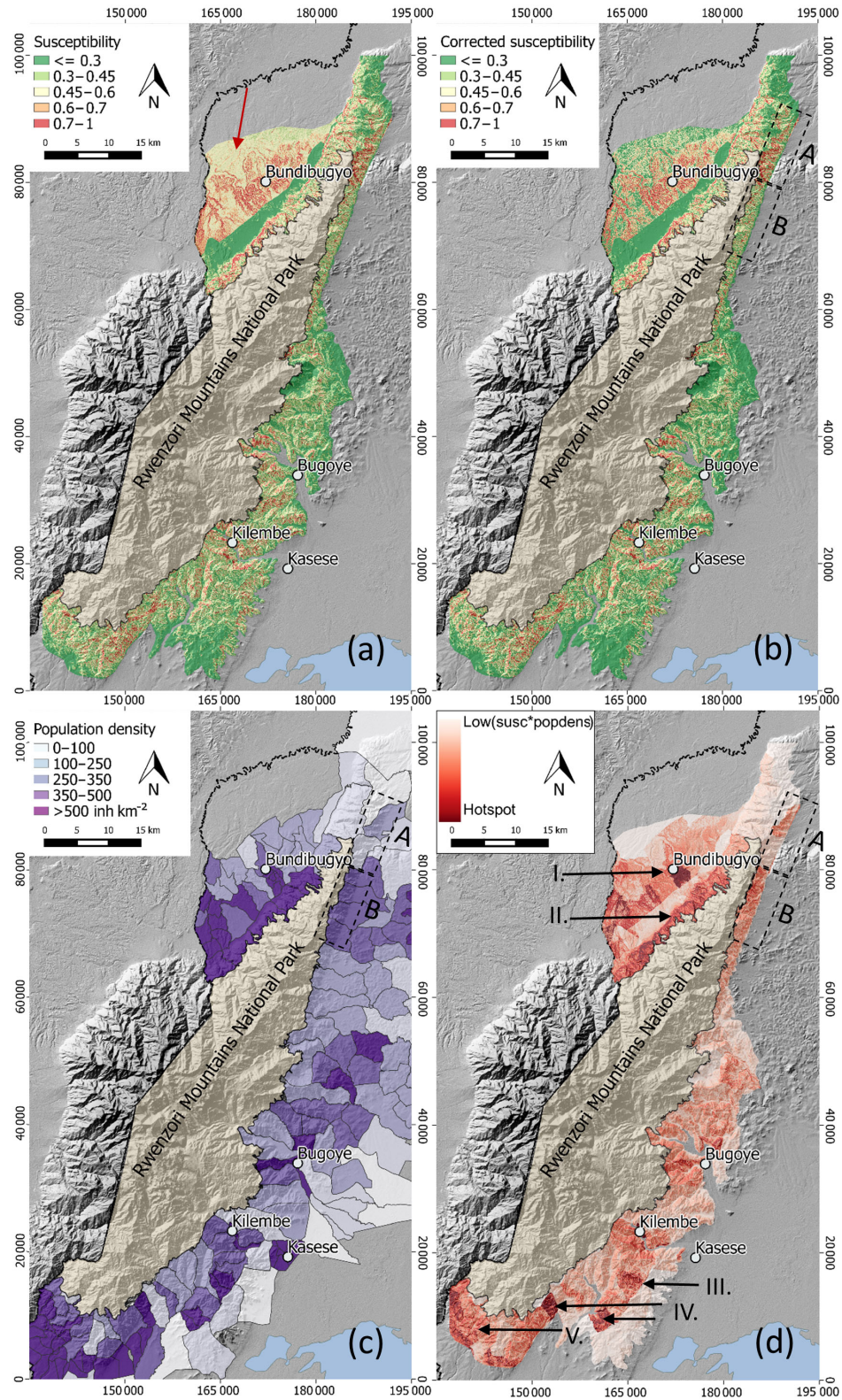
Figure 5. Landslide susceptibility ( susc ) and population density ( pop dens ) distribution in the Rwenzori Mountains’ inhabited zone. (a) Landslide susceptibility (red arrow indicates artefacts in regional landslide susceptibility model). (b) Corrected landslide susceptibility. (c) Population density at parish level (source: UBOS, 2003). (d) Preliminary identification of landslide hotspots. A and B indicate polygons discussed in the text. I to V indicate particular hotspot locations elaborated in the text.
