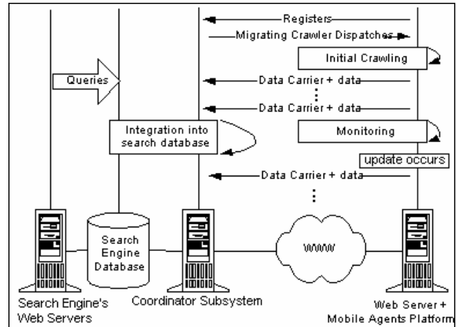
Figure 2. UCYMicra at work.
