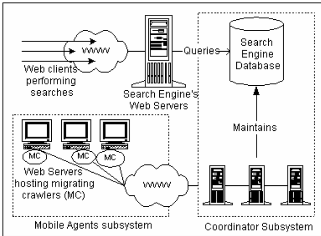
Figure 1. UCYMicra's Architecture.
