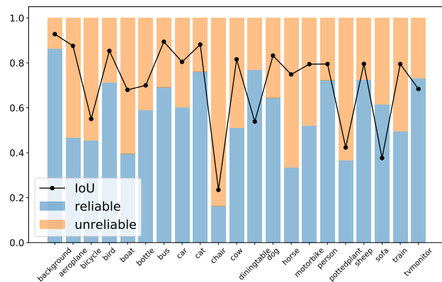
Figure 1. Category-wise performance and statistics on number of pixels with reliable and unreliable predictions. Model is trained using 732 labeled images on PASCAL VOC 2012 [16] and evaluated on the remaining 9,850 images.
