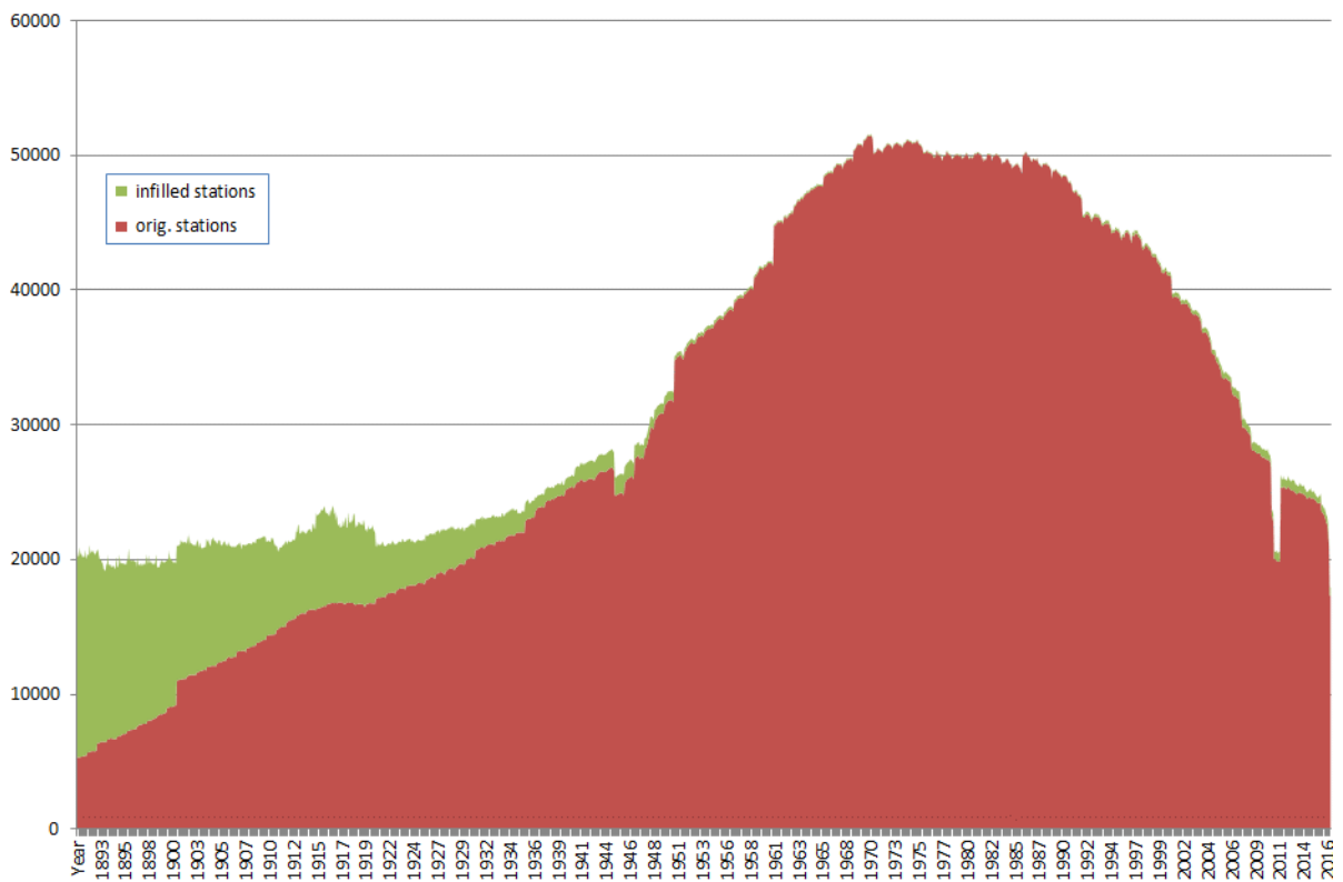
Figure 1: Number of monthly precipitation data over time since 1891 for GPCC's Full Data Monthly Analysis V.2018 (V.8) from original stations and added by climatological infilling
