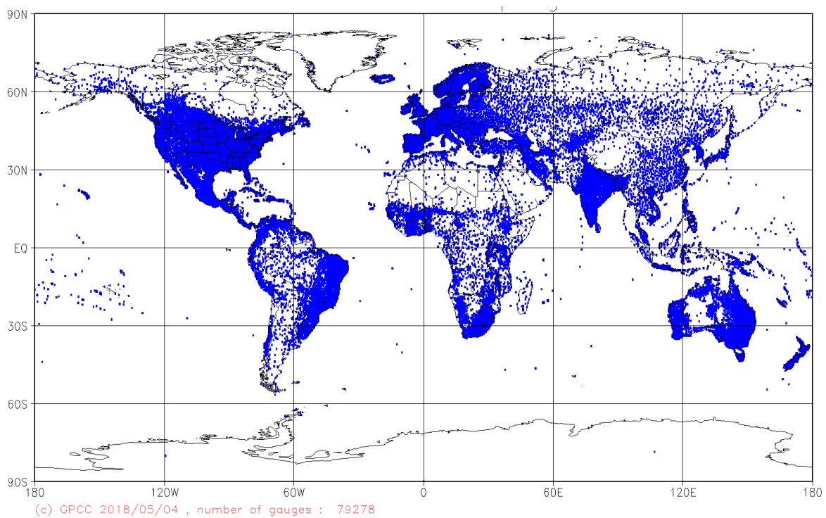
Figure 10: Spatial distribution of monthly in-situ stations with a climatological precipitation normal, based on at least 10 years of data in GPCCC's data base (number of stations in July: 79,278)
