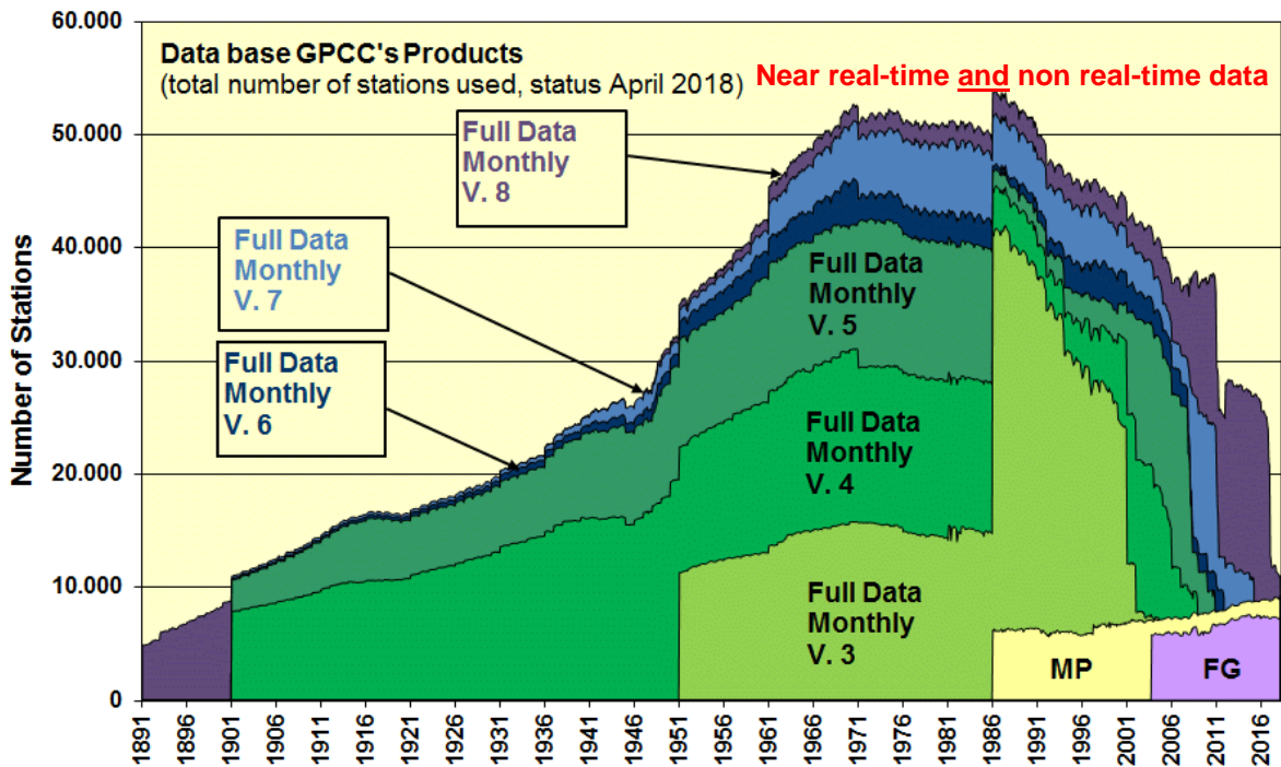
Figure 7: Total number of stations used for the GPCC products (Near real-time First-Guess Monthly Product "FG", Monitoring Product "MP"; non real-time Full Data Monthly Product (Versions 3 to 8))
