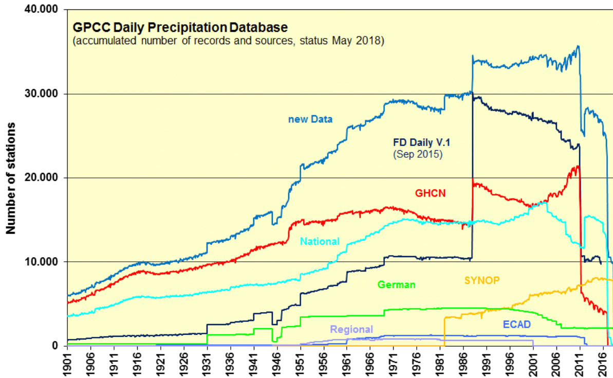
Figure 9: Total number of stations with daily precipitation data in GPCCC's full data base according to the different data sources
