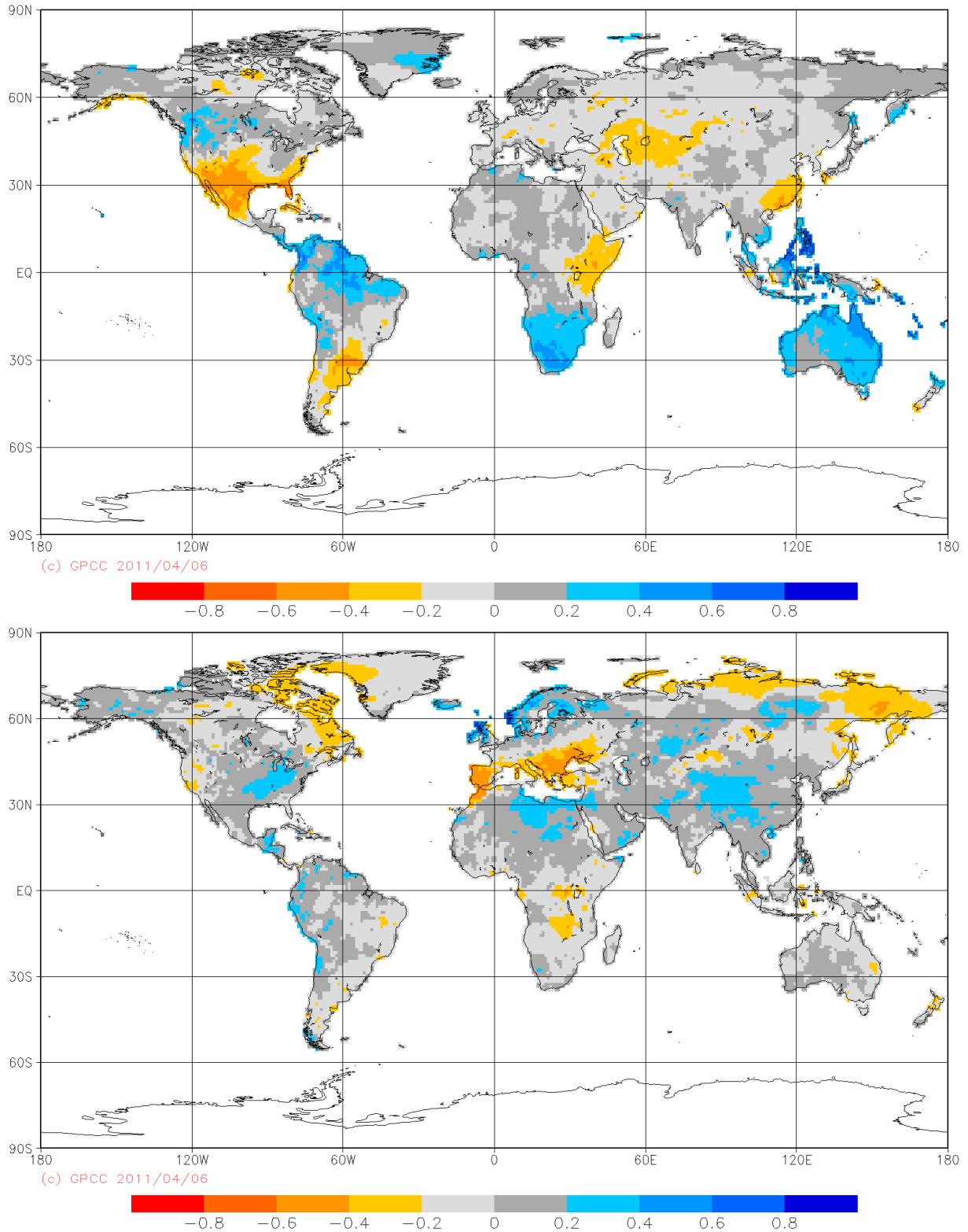
Figure 6: Correlation between monthly time series of gridded precipitation anomalies for the period 1901-March 2011 and (top) SOI and (bottom) NAO index (based on GPCP Full Data Monthly V.5, 0.5° resolution, since Jan. 2010 Monitoring Product V.3)
