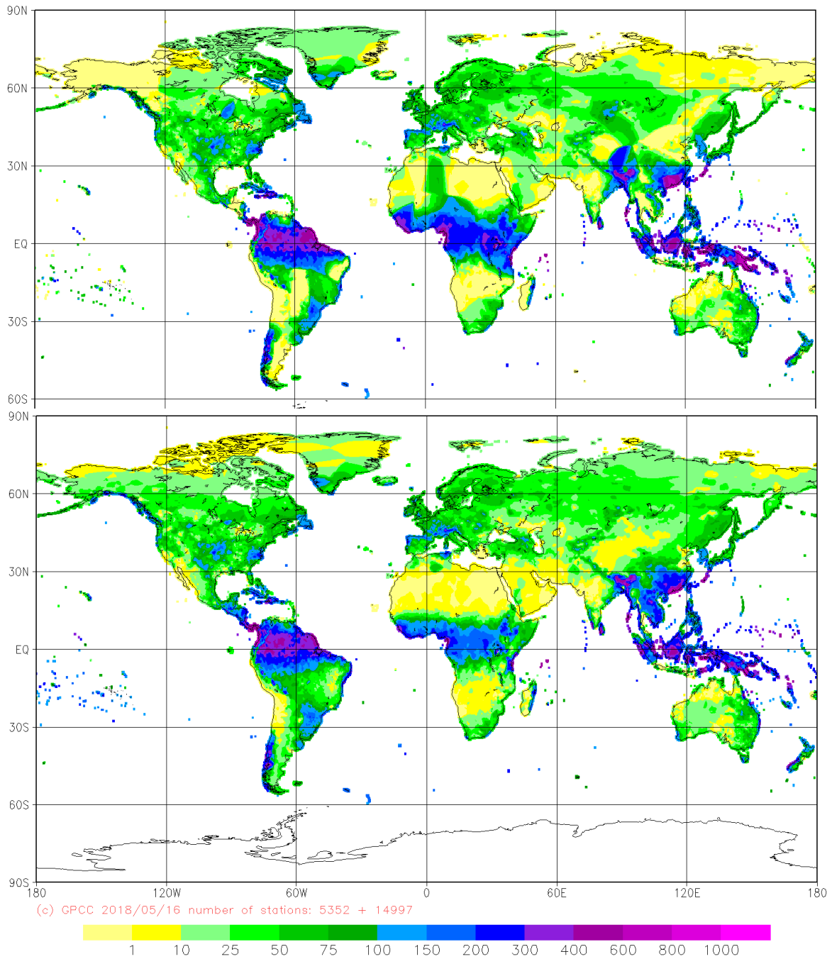
Figure 2: GPCP's Full Data Monthly Analysis V.2018 for May 1891 (top) without and (bottom) with climatological infilling
