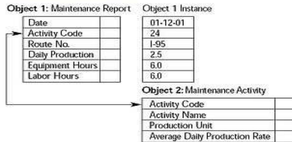
Figure 2.3: Object-oriented model [1]
