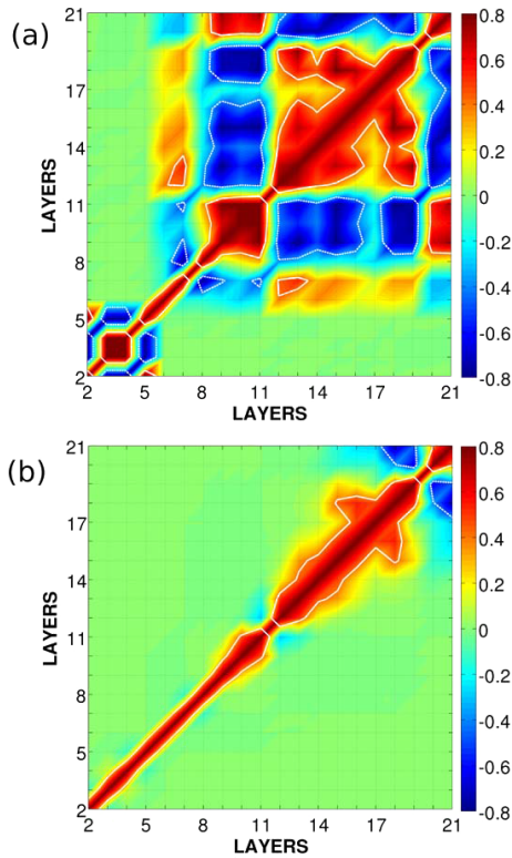
Figure 3. Vertical correlations of layer thickness between different layers at the location of an Argo float ( 69.95^\circ W and 30.14^\circ N) in the model domain: (a) calculated directly from the model ensembles ( M = 132 ) and (b) after applying the vertical localization of layer thickness according to Eq. (5) and L_\rho defined as 0.5 \text{ kg m}^{-3} . The white lines denote correlations above 0.4 and below -0.4 .
