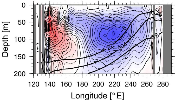
(a) W reg. Nino3, NEW
