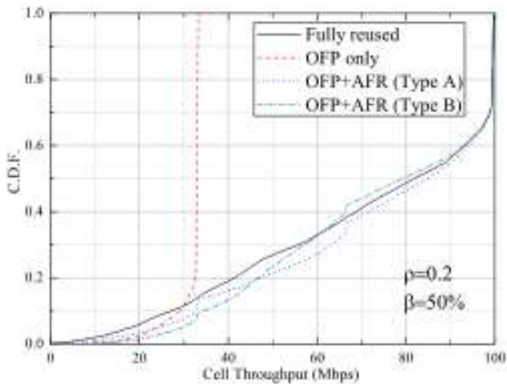
Fig. 15: Representation of CDF vs cell throughput (Zheng et al. , 2010)
