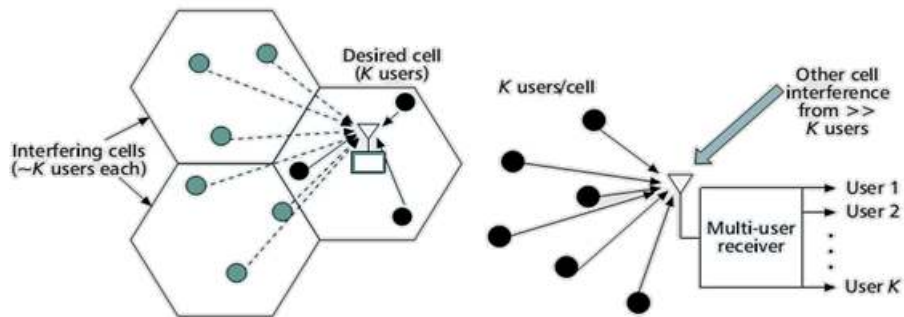
Fig. 11: Uplink interference scenarios (Andrews, 2005)
