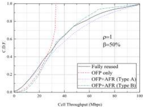
Fig. 16: Illustration of CDF vs. cell throughput with \rho = 1 and \beta = 50\% (Zheng et al. , 2010)
