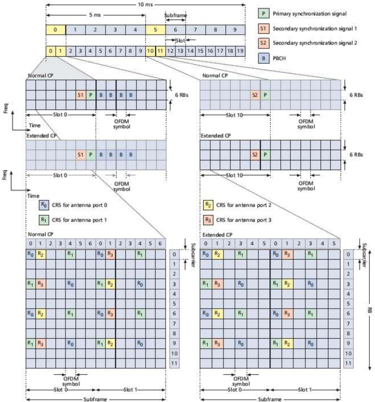
Fig. 3: Illustration of for OFDMA DL physical layer arrangement (Aleksandar et al. , 2011)
