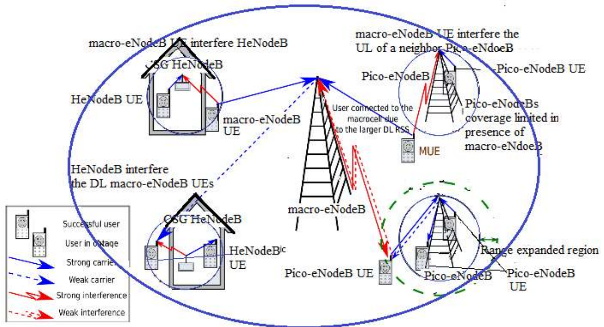
Fig. 9: Representation of UL/DL cross-tier interference scenarios in HetNet
