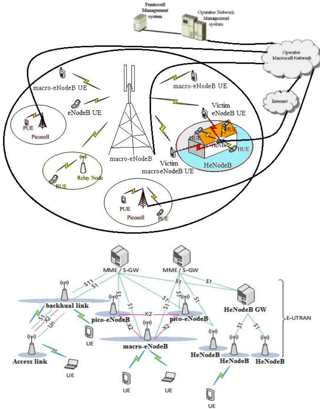
Fig. 1: LTE-A HetNet network architecture with the interfaces (Aleksandar et al. , 2011)
