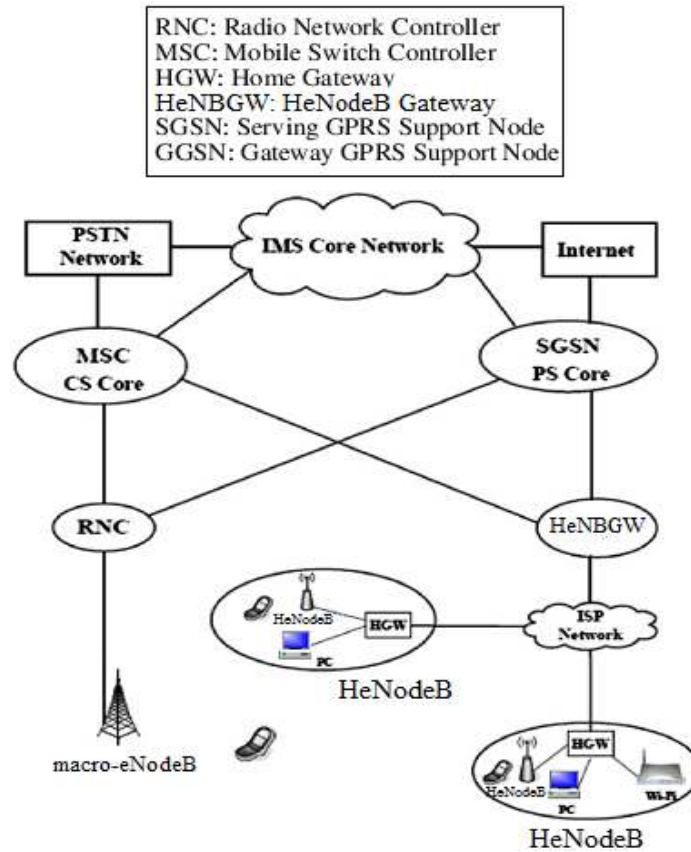
Fig. 5: The deployment of HeNodeB in SON (David, 2009)
