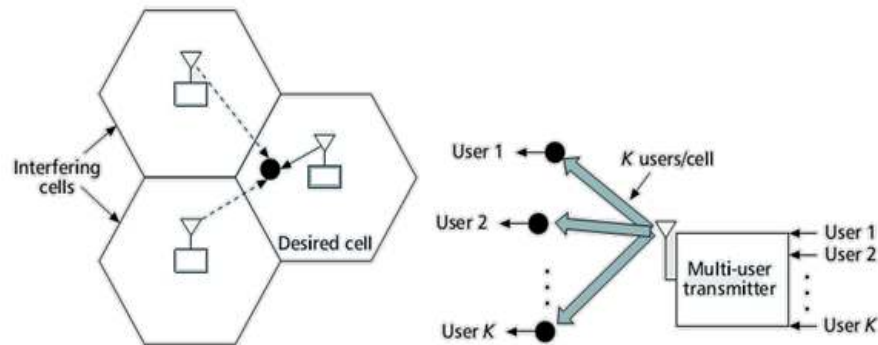
Fig. 10: Downlink interference scenario (Andrews, 2005)
