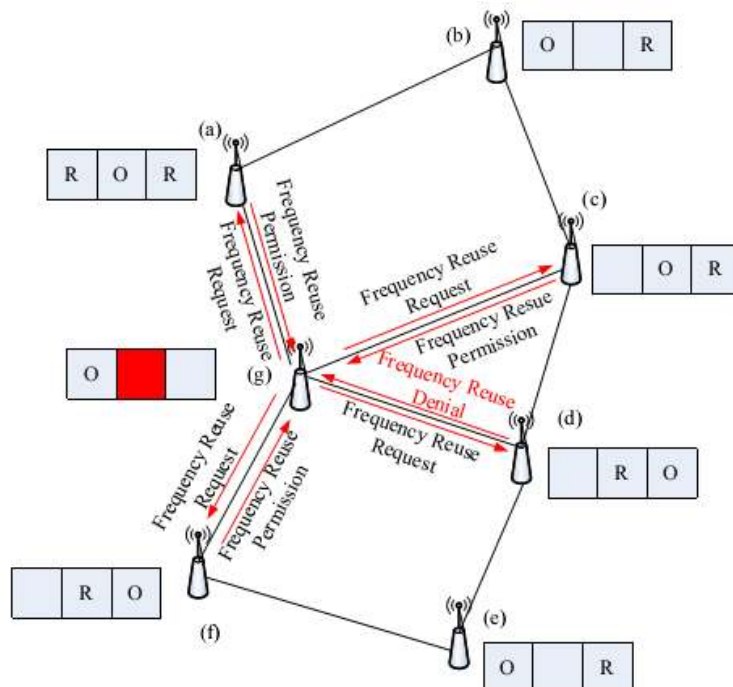
Fig. 13: Illustration of adaptive frequency reuse process (Zheng et al. , 2010)
