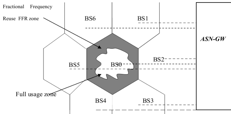
Fig. 12: AFFR system model (Suzan et al. , 2009)
