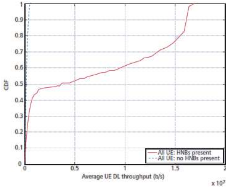
Fig. 7: DL user throughput distributions on shared frequency (Mehmet et al. , 2009)
