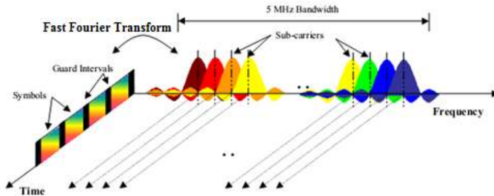
Fig. 2: Frequency-time illustration of an OFDM signal (Erik et al. , 2011)
