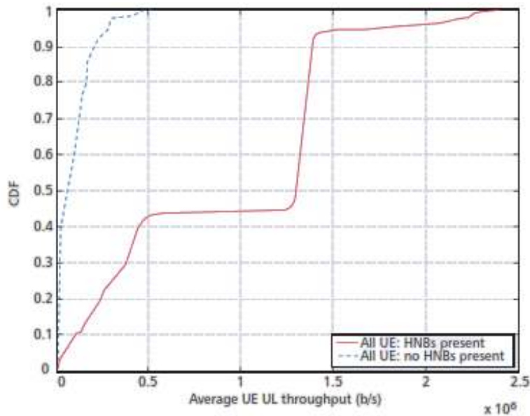
Fig. 8: UL user throughput distributions on shared frequency (Mehmet et al. , 2009)
