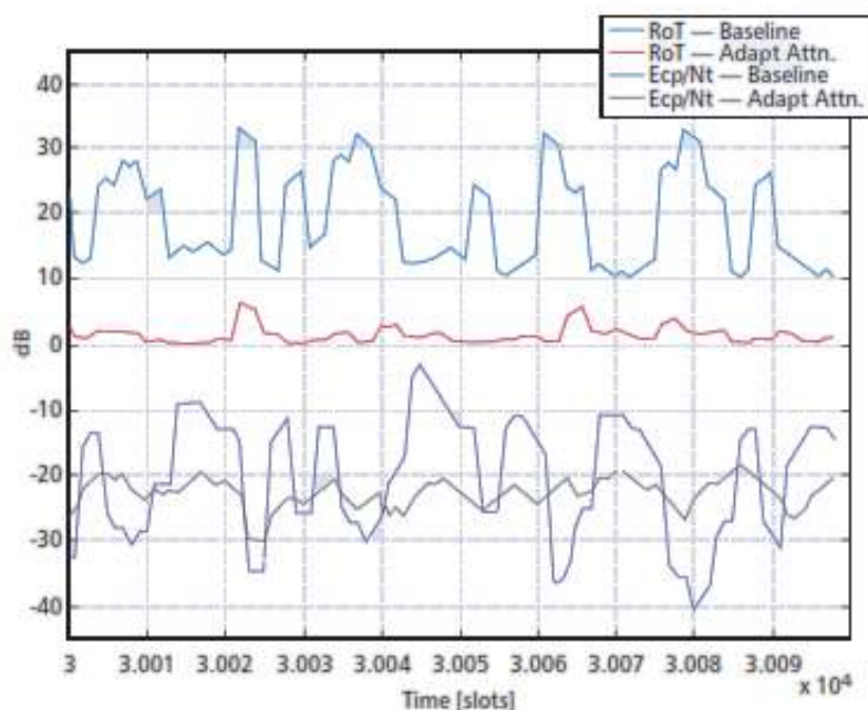
Fig. 6: Interference performance of HeNodeB UL (Mehmet et al. , 2009)
