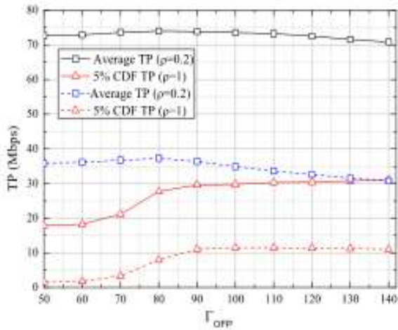
Fig. 14: Throughput performances with different threshold (Zheng et al. , 2010)
