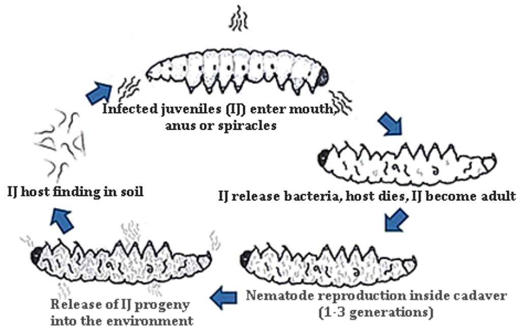
Figure 1. Entomopathogenic nematode lifecycle (Tofangsazi et al. , 2012).
