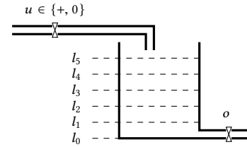
Figure 1: Tank reactor modeled as a dynamical system S over an infinite bounded state space X \subset \mathbb{R}^3 with finite input space U = \{+, 0\} and finite output space Y \subseteq 2^\sigma denoting the set of sensors \sigma = \{l_0, \dots, l_5, o\} which are currently ‘true.’
