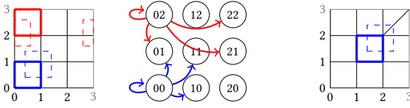
Figure 5: Graphical representation of \Sigma_1 (far left) and \Sigma_2 (far right), showing the state space X with the partition induced by the output maps H_1 and H_2 , respectively. For \Sigma_1 , X_j = F(X_i, u_1) (dashed blue) indicates the reachable set of X_i = H_1^{-1}(y_{00}) (solid blue). Intersecting X_j with the partition generates transitions (blue) originating in y_{00} in the finite-state abstraction (middle). Similarly, X_j = F(X_i, u_2) (dashed red) is reached from X_i = H_1^{-1}(y_{02}) (solid red) generating transitions (red) originating in y_{02} in the abstraction.
