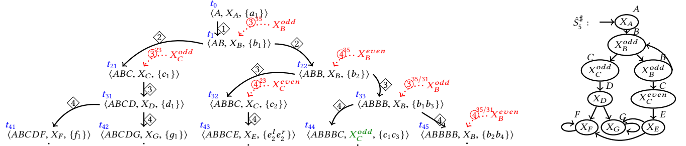
Figure 4: Exploration tree \text{EXP}_F of S in Fig. 3 computed by Alg. 2 (left) and the abstract system \hat{S}^\# extracted after its 5th iteration (right). Nodes are labeled by t_k (blue) for easier reference and the single input u is omitted to avoid clutter. Diamond-enclosed numbers indicate the iteration in which this transition is explored. Dotted red arcs indicate cover block refinements in the iteration of the main while loop depicted by the red circled number and caused by the line of REFINE indicated on its top right. E.g., X_B of t_1 is refined by re-calling REFINE in line 35 after X_C of t_{21} was refined in line 23 (as t_1 is a predecessor of t_{21} ). The notation 35/31 in t_{45} indicates that its cover block X_B is refined by line 31 after re-calling REFINE via line 35 on node t_{22} .
