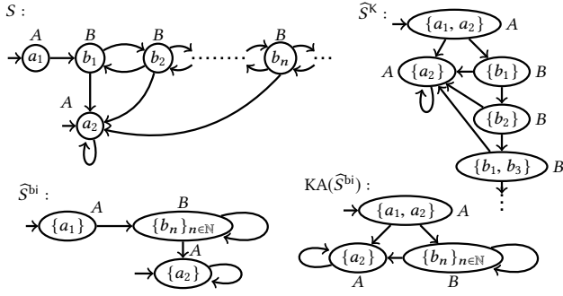
Figure 2: The system S (top left) has an infinite-state knowledge abstraction \widehat{S}^K (top right) while an exact finite-state representation of \text{Ext}(S) exists, which is correctly computed by first computing the bisimilarity abstraction \widehat{S}^{bi} (bottom left, see Sec. 4.2) and then applying Alg. 1 (bottom right).
