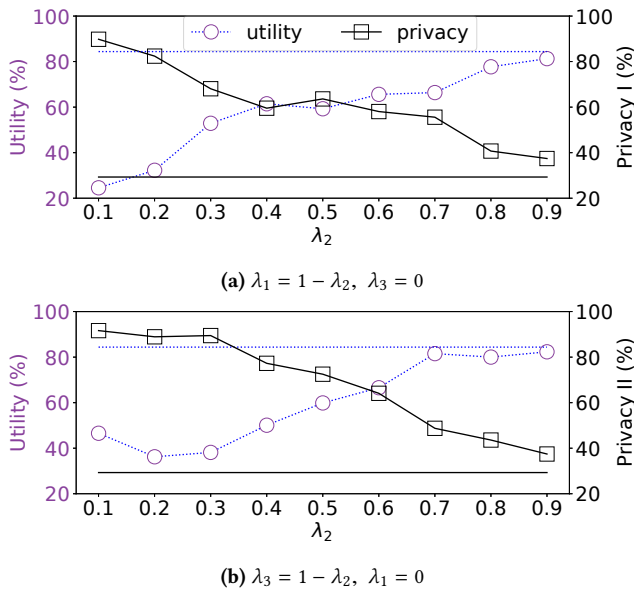
Figure 7: Varying weights can tune the privacy-utility trade-offs. The primary y-axis (dashed line) represents utility, and the secondary y-axis (solid line) represents privacy. The x-axis represents the value of the target \lambda .
