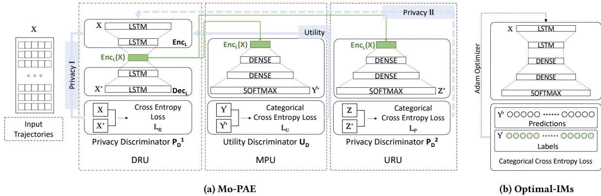
Figure 2: (a) Schematic overview of the proposed privacy-preserving adversarial architecture (Mo-PAE), consisting of data reconstruction risk unit (DRU), mobility prediction unit (MPU), and user re-identification risk unit (URU); (b) The baseline LSTM network for optimal classifiers (Optimal-IMs).
