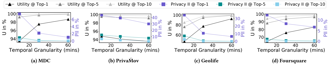
Figure 5: The effect of temporal granularity on the model performance of four mobility datasets.
