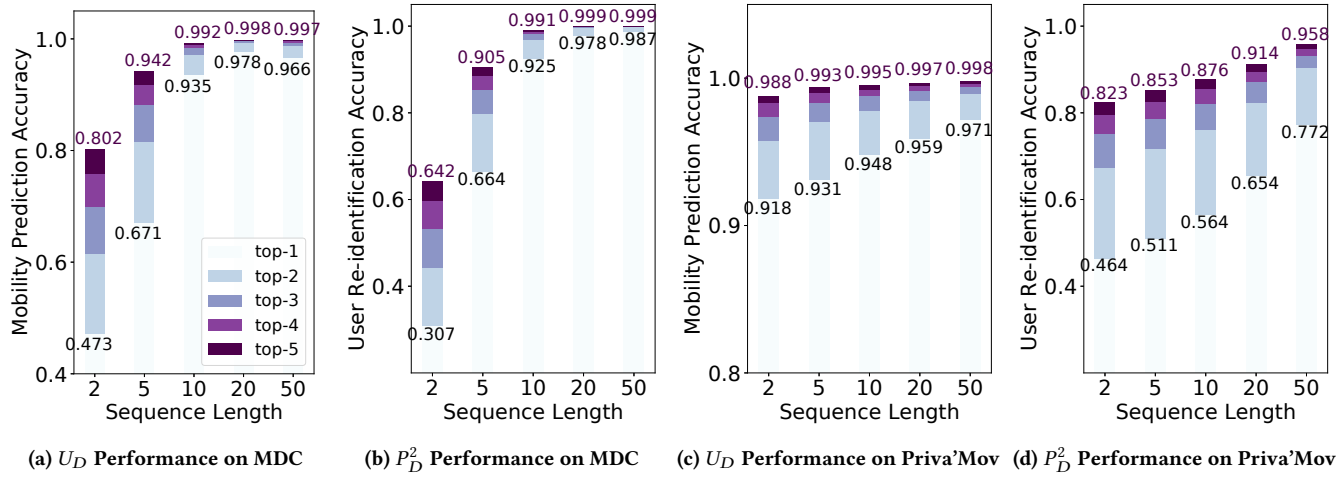
Figure 6: Mobility prediction accuracy and user re-identification accuracy change with the trace sequence length (SL) in our proposed U_D and P_D^2 . The color bars indicate the accuracy from top-1 to top-5, the black texts indicate the top-1 accuracy, and the purple texts indicate the top-5 accuracy. For instance, the top-1 mobility prediction accuracy on MDC with SL = 2 is 0.473, and the top-5 one is 0.802.
