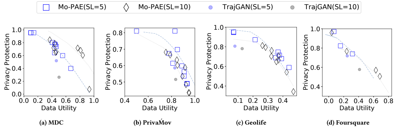
Figure 3: Pareto Frontier trade-off analysis on four datasets. The hollow squares and diamonds present the results of the proposed models Mo-PAE. solid points present the results of the TrajGAN. Blue color means SL = 5 . Black color means SL = 10 .
