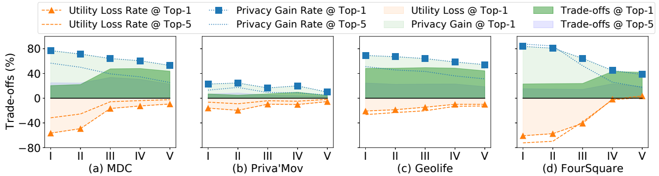
Figure 4: Impact of Mo-PAE on the user re-identification accuracy (PII) and relative utility loss (U) on four datasets. The orange area represents the utility loss, while the light-green area represents privacy gain. The dark-green area represents the trade-offs between utility achievement and privacy budgets. The x-axis shows five different model settings, and the y-axis shows the trade-offs.
