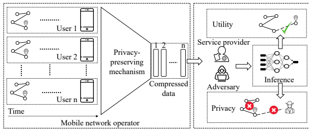
Figure 1: Privacy protection in user's location data collection and sharing. Users share their daily traces to a trusted mobile network operator; these traces are aggregated with a privacy-preserving mechanism and shared as a compressed data format; the compressed data should allow utility inference and avoid privacy inference.
