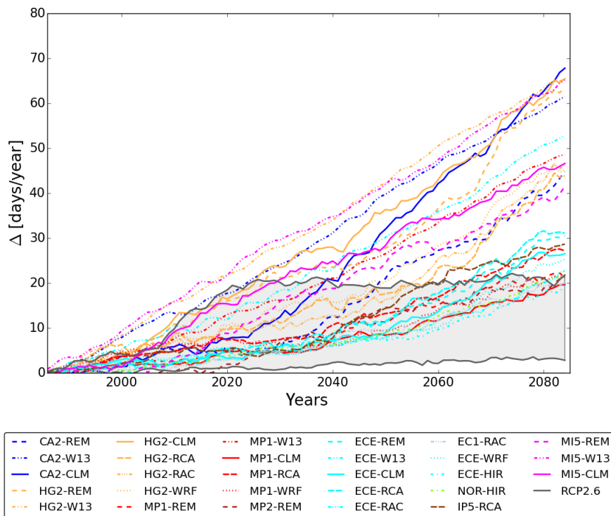
Figure 4. Change in number of summer days ( T_{\max} > 25\text{ }^{\circ}\text{C} ): The 30-year “running mean” 1986–2085 minus 1971–2000. The bandwidth between minimum and maximum change of the number of summer days is shown for RCP2.6 simulations in grey shading, the coloured lines show the changes calculated by simulations using RCP8.5.
