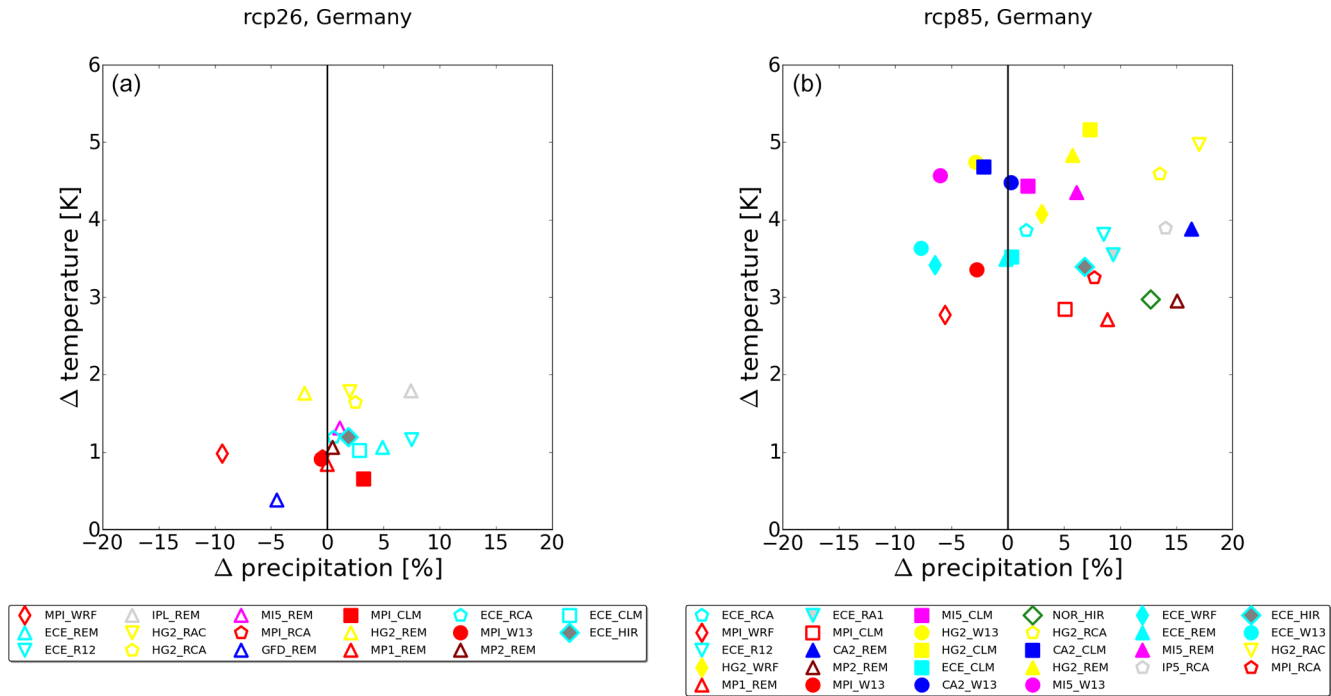
Figure 1. The mean annual change between 2071–2100 and 1971–2000 for temperature and precipitation of each model averaged over Germany (RCP2.6: a , RCP8.5: b ). The colour indicates the forcing GCM and each RCM has its specific symbol.
