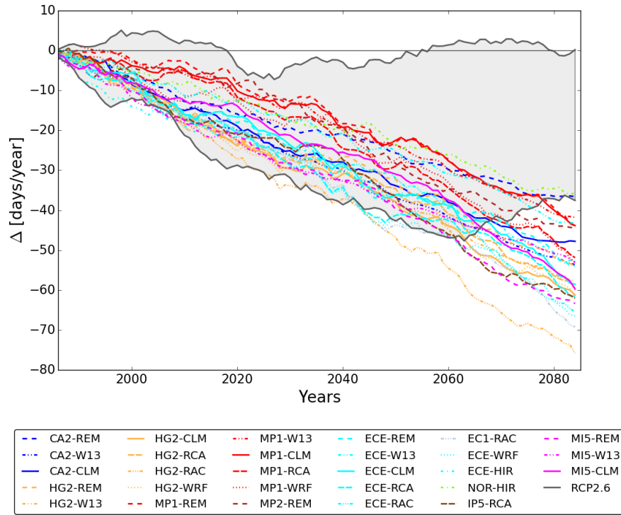
Figure 3. Change in number of frost days ( T_{\min} < 0\text{ }^{\circ}\text{C} ): The 30-year “running mean” 1986–2085 minus 1971–2000. The bandwidth between minimum and maximum change of the number of frost days is shown for RCP2.6 simulations in grey shading, the coloured lines show the changes calculated by simulations using RCP8.5.
