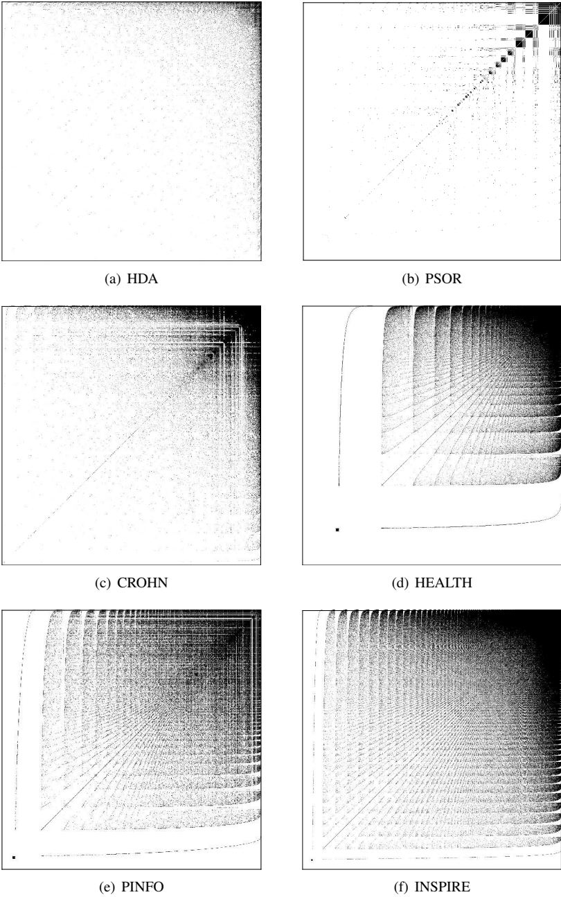
Figure 1. BOSAMs for the modelled networks. Node degree increases along the axes.
