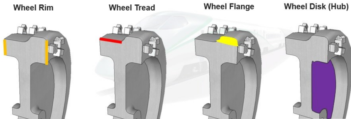
Critical wheel areas with their irregular surfaces
