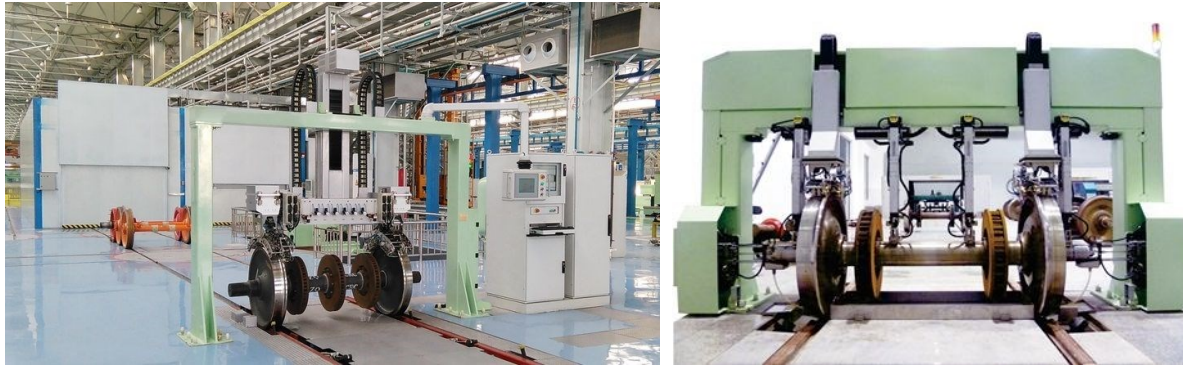
Dismounted wheelset and solid axle ultrasonic testing systems
