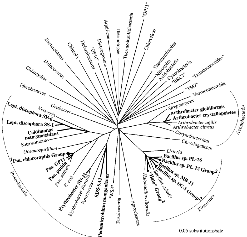
Figure 3 Location of Mn(II)-oxidizing bacteria on a neighbor-joining, unrooted phylogenetic tree of the Domain Bacteria. 16S rRNA sequences aligned over 1536 positions were obtained from the Ribosomal Database Project (RDP, http://rdp.cme.msu.edu ) and analyzed using PAUP (ver. 4.0b10). Mn(II)-oxidizing bacterial strains for which sequences appear in the RDP are shown in bold. Sequence similarity is only an estimate of evolutionary relationships and is expressed here as the distance between any two branch tips; sequences that appear next to each other are not necessarily close relatives. Phyla in quotes are considered taxa of uncertain affiliation and have few, if any, cultivated members. Abbreviations: Lept. , Leptothrix ; Psu. , Pseudomonas . 1 The Psu. chlororaphis group includes the Mn(II)-oxidizing strains ISO1, ISO6, GB-13, MG1, and PCP, but not all similarly close relatives of Psu. chlororaphis are known to oxidize Mn(II). 2 Bacillus species groups are labeled according to Francis & Tebo (2002).
