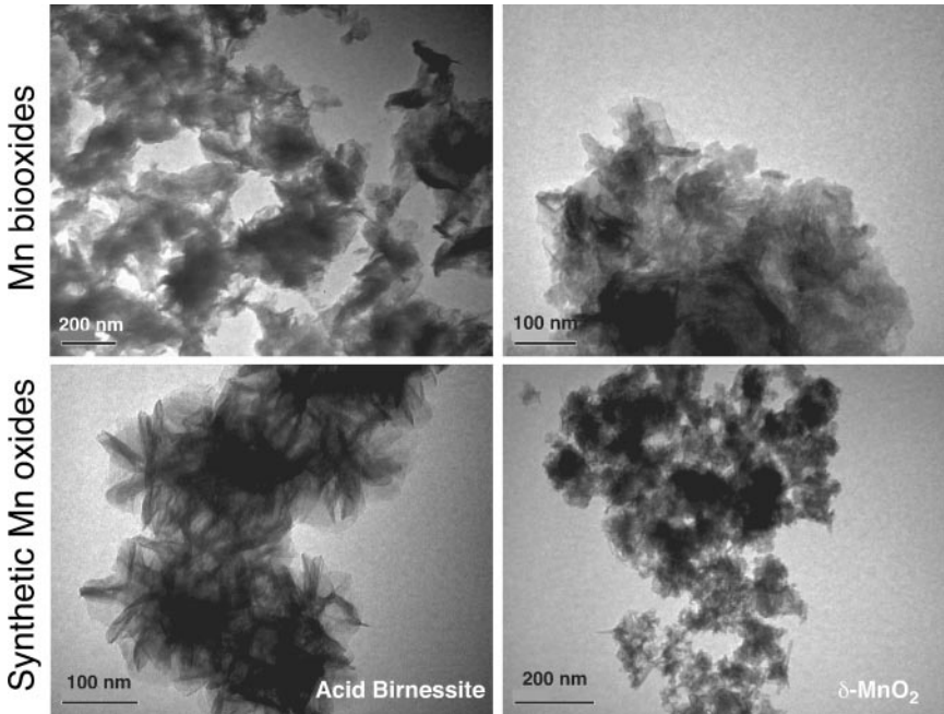
Figure 11 Transmission electron micrographs of synthetic Mn oxides ( lower panels ) and the Mn biooxide produced by P. putida strain Mn-B1 ( upper panels ). Reprinted from Villalobos et al. (2003), with permission from Elsevier.
