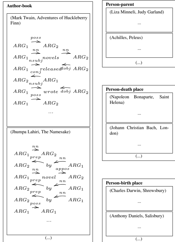
Figure 1: Example of a generated set of document collections from a news corpus for relation extraction. Larger boxes are document collections (relations), and inner boxes are documents (entity pairs). Document contain dependency patterns, which are words in the topic model.
