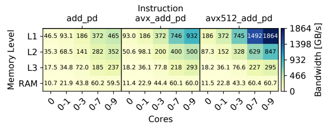
Figure 10: Intel Xeon Gold 6248 – bandwidth at nominal AVX-512 frequency (1.6 GHz) for one SNC
