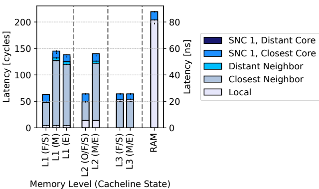
Figure 15: Memory read latencies for an Intel Xeon Gold 6248 on one socket, measured from SNC 0 – Forwarded and Shared states result in identical latencies, Modified and Exclusive latencies only for L2 and L3. Refer Table 3 for precise values.
