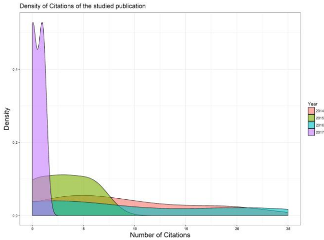
Figure 3. Density plot of citations per year
