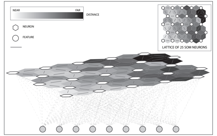
Fig. 3. Typical visualisation of Self Organizing Maps
