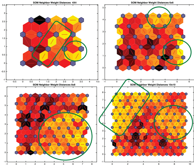
Fig. 5. SOM neighbor distances for 4 different neuron lattices. The light coloured distances correspond to the created cluster of neurons in a neighbourhood.
