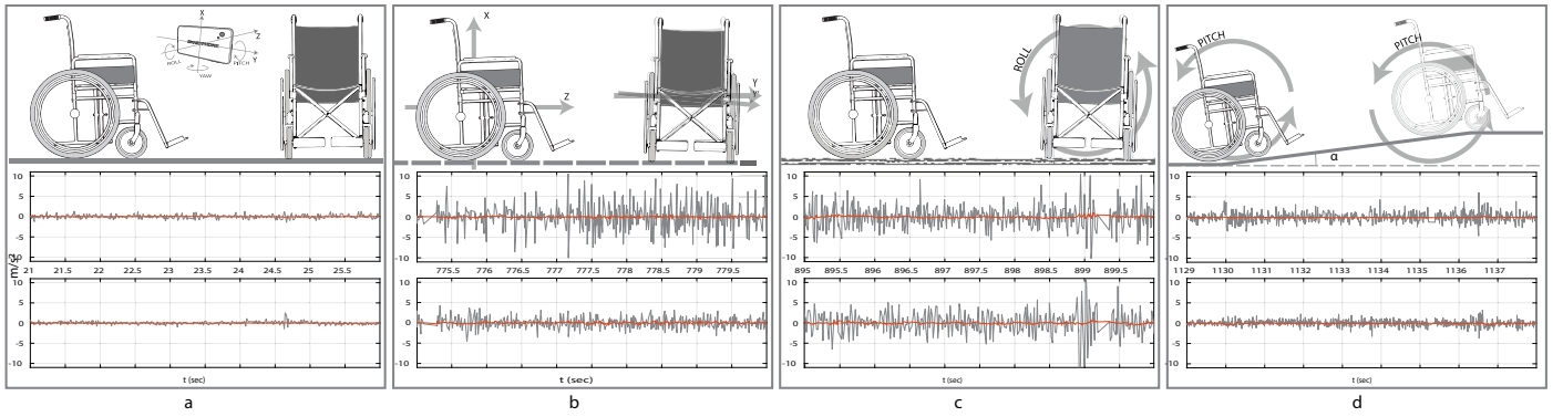
Fig. 2. Wheelchair measurements over different type of surfaces. Wheelchair a) riding a smooth indoor surface, b) riding tiled with big gaps pavement, c) riding an unpaved but well pressed gravel pavement, d) entering a ramp
