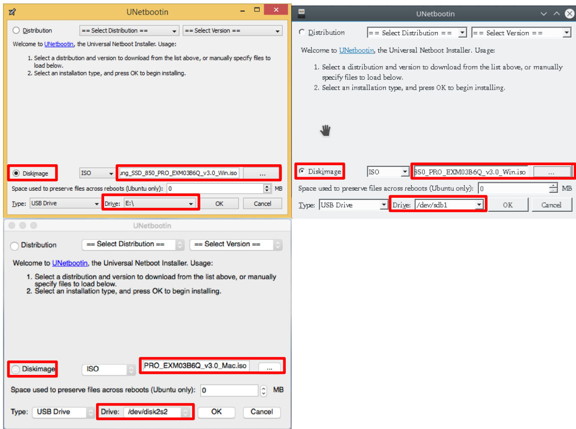
Figure 1. UNetbootin (Windows, Linux, Mac)
