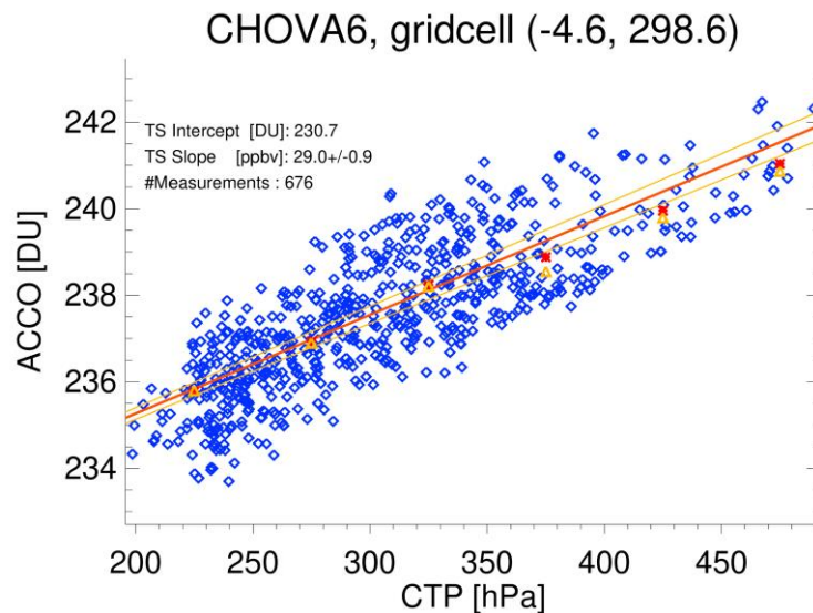
Figure 5.4: TROPOMI tropical tropospheric ozone volume mixing ratios [ppbv] calculated from the slope of the Theil-Sen regression between above-cloud ozone and cloud-top-pressure. The regression here is limited to ACCOs for cloud top pressures less than 500 hPa. The grid box size is 3° and the time span for collection is one day.
