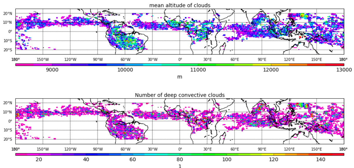
Figure 7.1: Mean altitude and occurrence of deep-convective clouds as derived from Sentinel-5p oxygen A band measurements using the OCRA/ROCINN algorithm. Results are shown for 2018 October 26 th to 31 st . Clouds are classified as deep convective if their tops are above 8.5 km, the cloud albedo larger than 0.8, and their cloud fraction exceeds 0.8.
