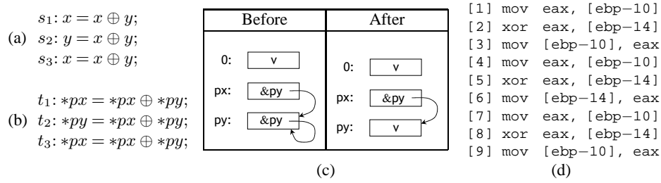
Fig. 1. (a) Code fragment that swaps two ints ; (b) code fragment that swaps two ints using pointers; (c) possible before and after configurations for code fragment (b): the swap is unsuccessful due to aliasing; (d) x86 machine code corresponding to (a).
