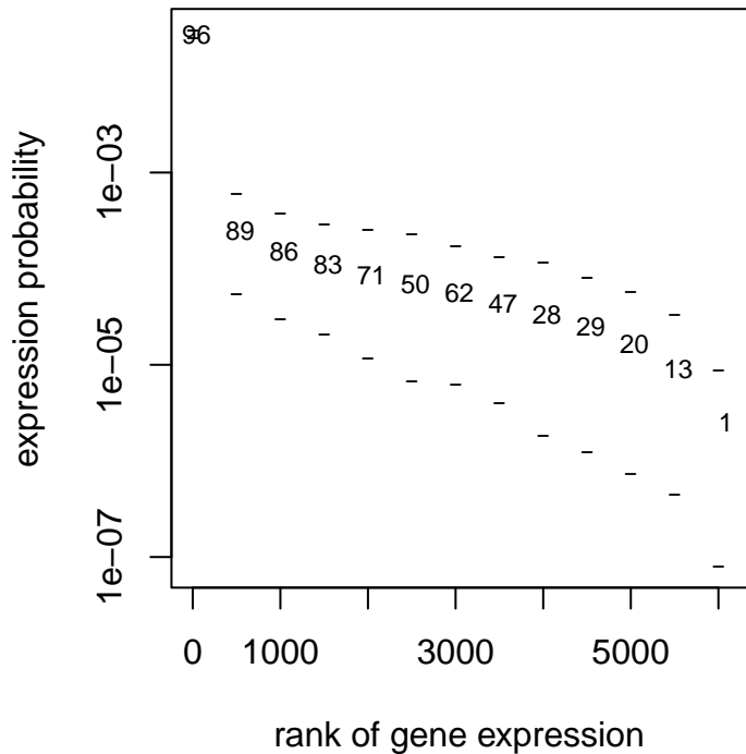
Tub prior
