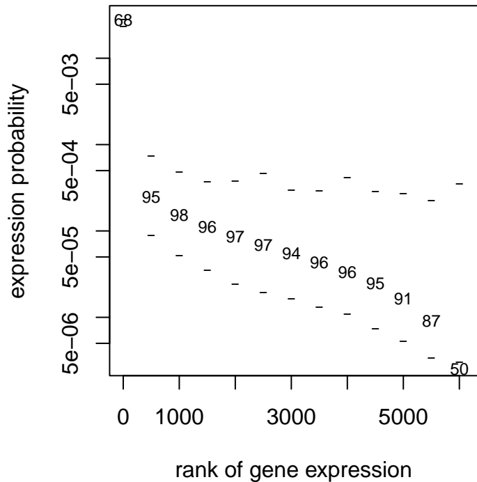
Flat prior
