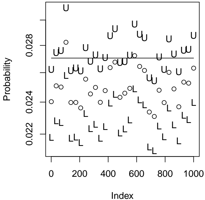
Gene2 Flat Prior
