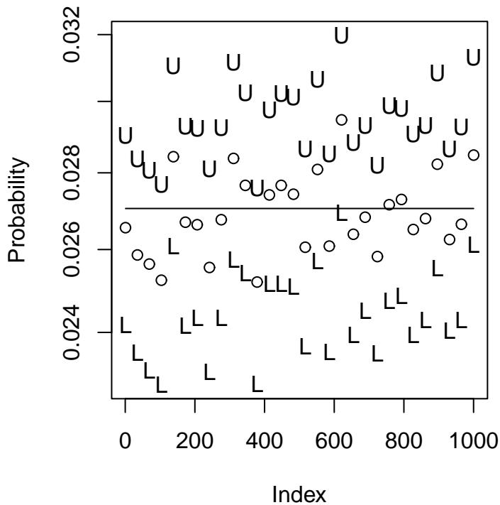
Gene2 Tub Prior
