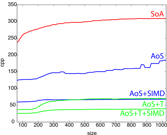
HaswellIM+SSE
