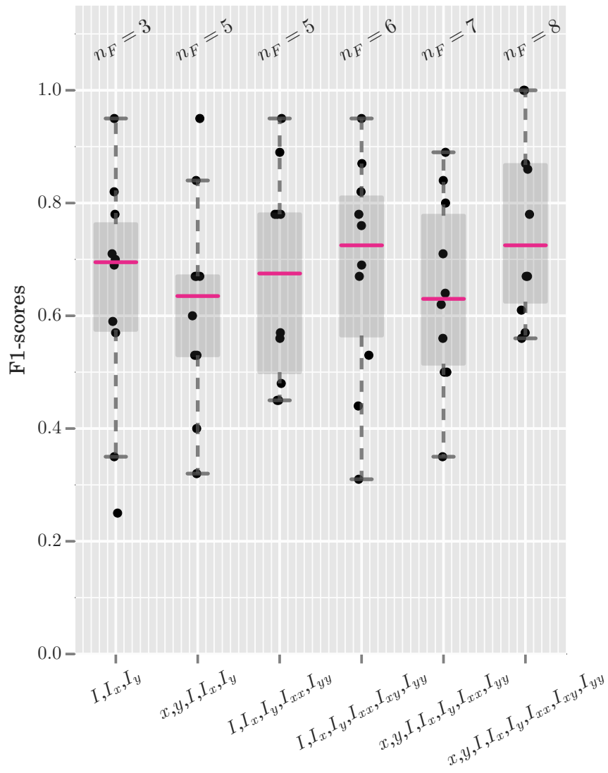
Evaluation with KTH-Tips dataset (gradients)
