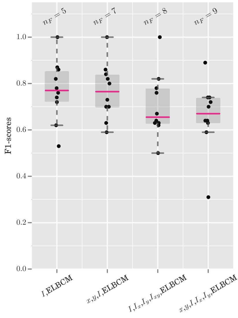
Evaluation with KTH-Tips dataset (ELBCM)
