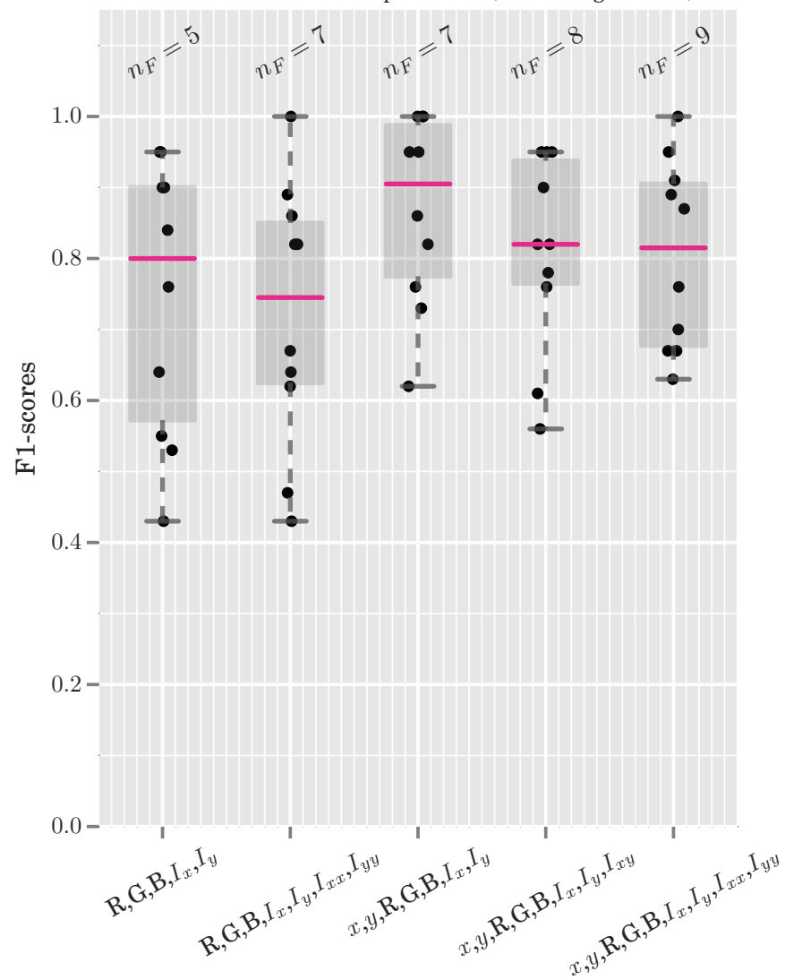
Evaluation with KTH-Tips dataset (color and gradients)
