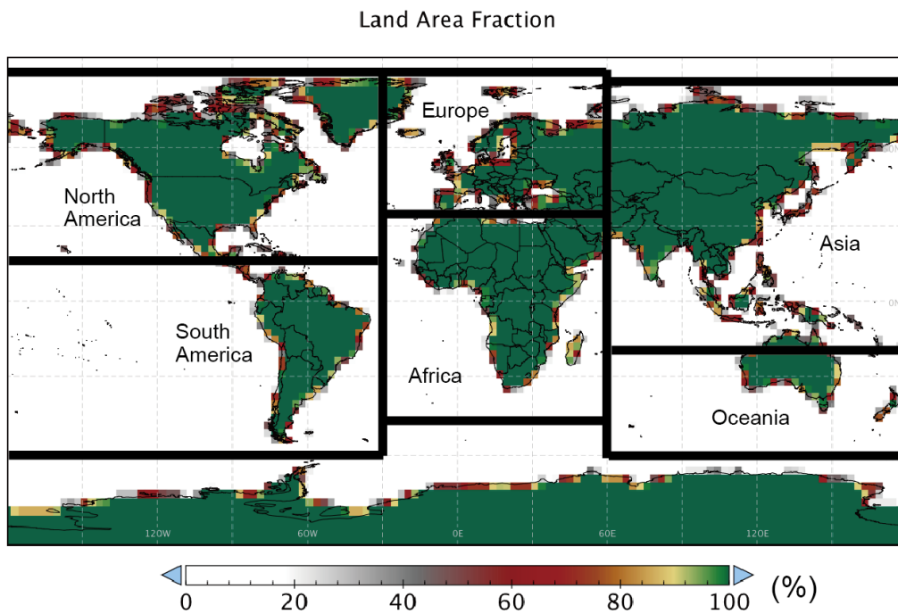
Fig. S2 Regional boundaries used in this study overlaid on the MIROC-ES2L land fraction map: Asia (856 land grids, 41.7 \times 10^6 km 2 ), Africa (462 land grids, 35.9 \times 10^6 km 2 ), Oceania (112 land grids, 7.0 \times 10^6 km 2 ), Europe (347 land grids, 13.6 \times 10^6 km 2 ), North America (653 land grids, 25.2 \times 10^6 km 2 ), and South America (271 land grids, 18.7 \times 10^6 km 2 )
