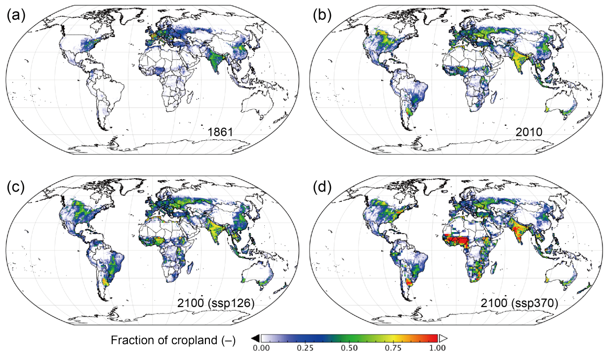
Fig. S3 Changes in the cropland fraction in (a) 1861, (b) 2010, (c) 2100 by ssp126, and (d) 2100 by ssp370. Data were derived by using Land Use Harmonization version 2
