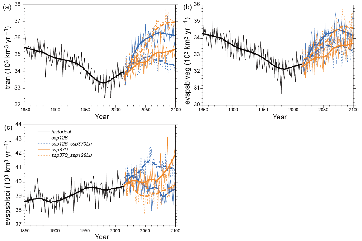
Fig. S5 Temporal changes in global water flows. (a) Vegetation transpiration (tran), (b) evaporation from canopy-intercepted precipitation (evspsblveg), and (c) evaporation from soil (evspsblsoi)
