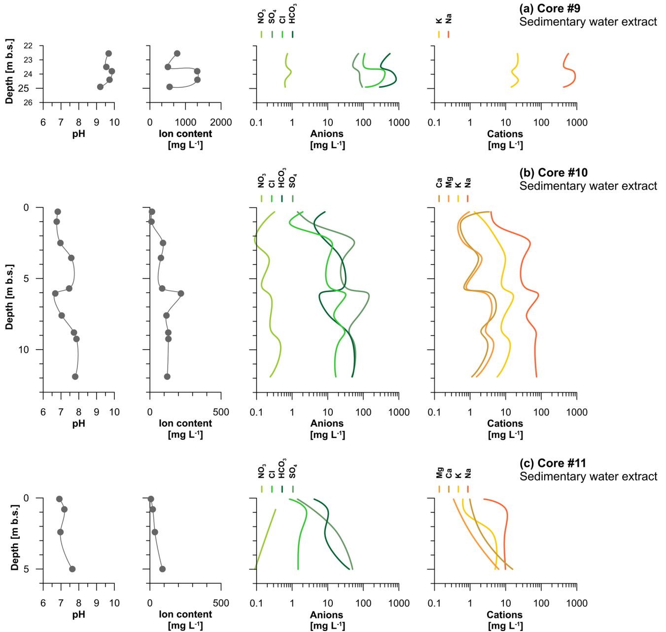
Figure 4. Hydrochemical composition of water extracts from the sedimentary cores 9, 10 and 11. Data are given in Table 3. Note different axis scale for ion content in (a) reaching up to 1335 \text{ mg L}^{-1} .
