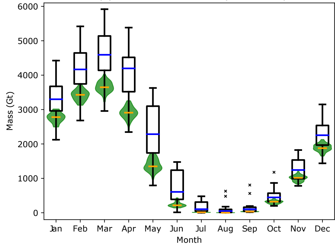
(b) CMIP6 NH snow mass (1981–2014)
