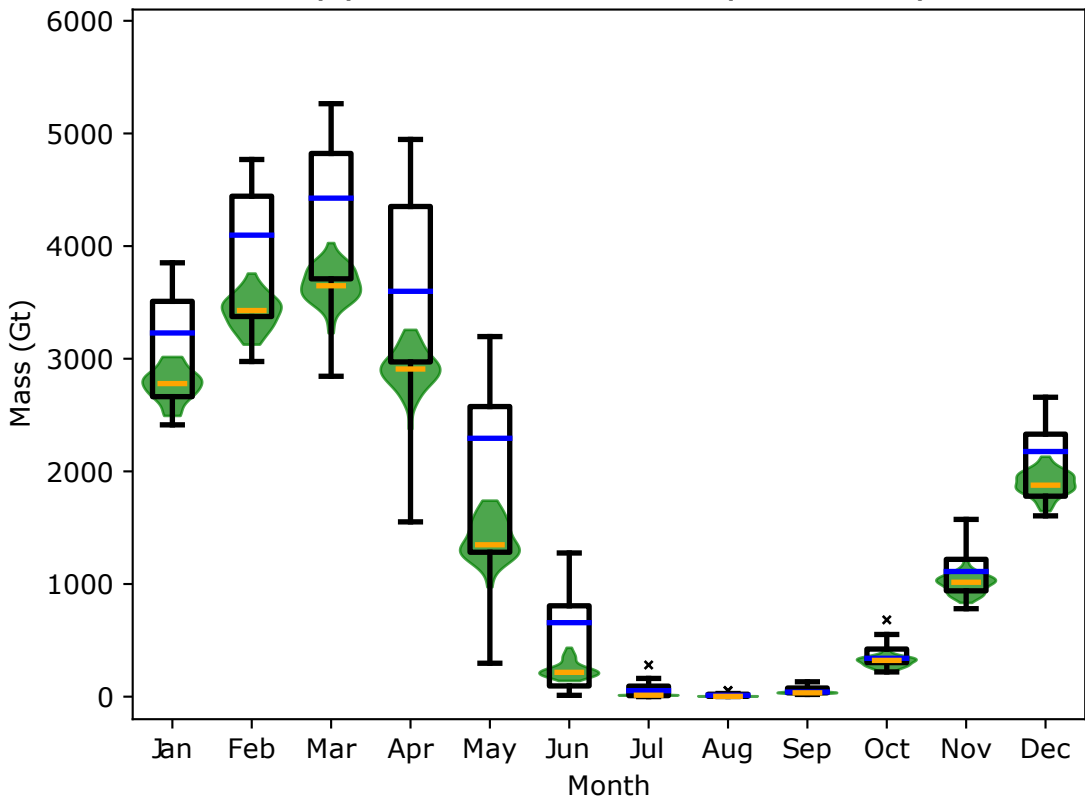
(a) CMIP5 NH snow mass (1981–2014)
